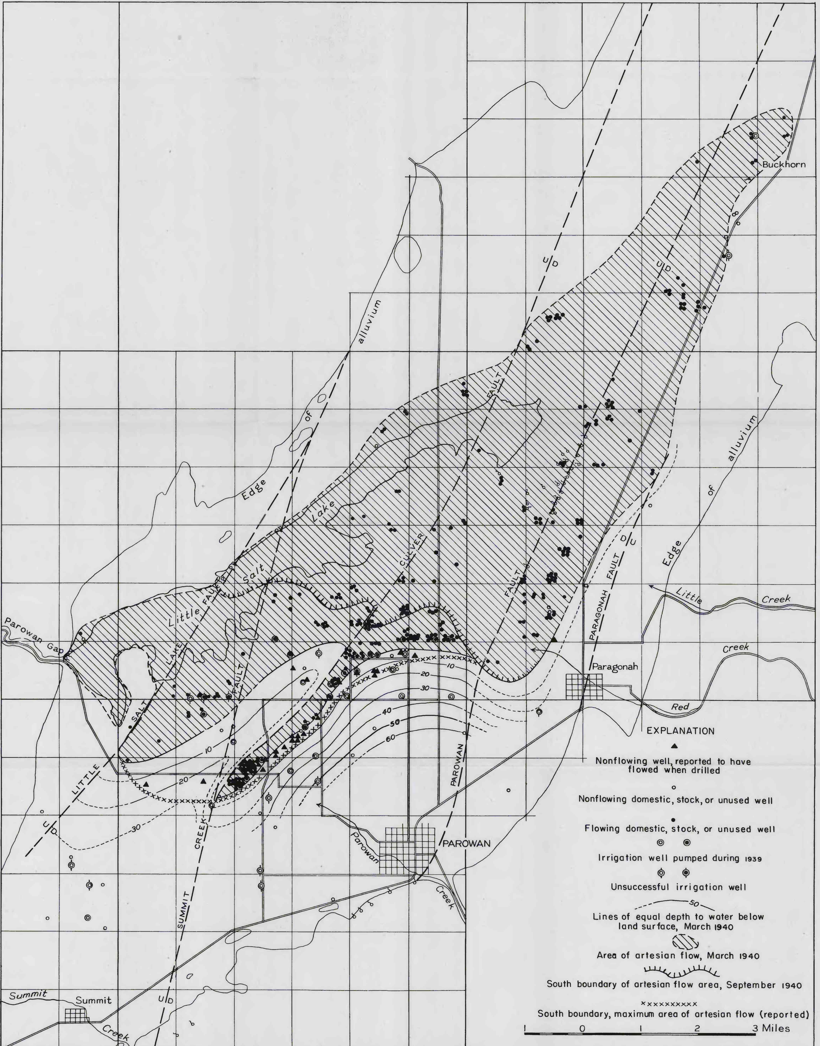
MAP OF PAROWAN VALLEY SHOWING LOCATION OF WELLS AND SPRINGS AND POSITION OF HIGHEST PIEZOMETRIC SURFACE WITH RESPECT TO LAND SURFACE IN 1940
