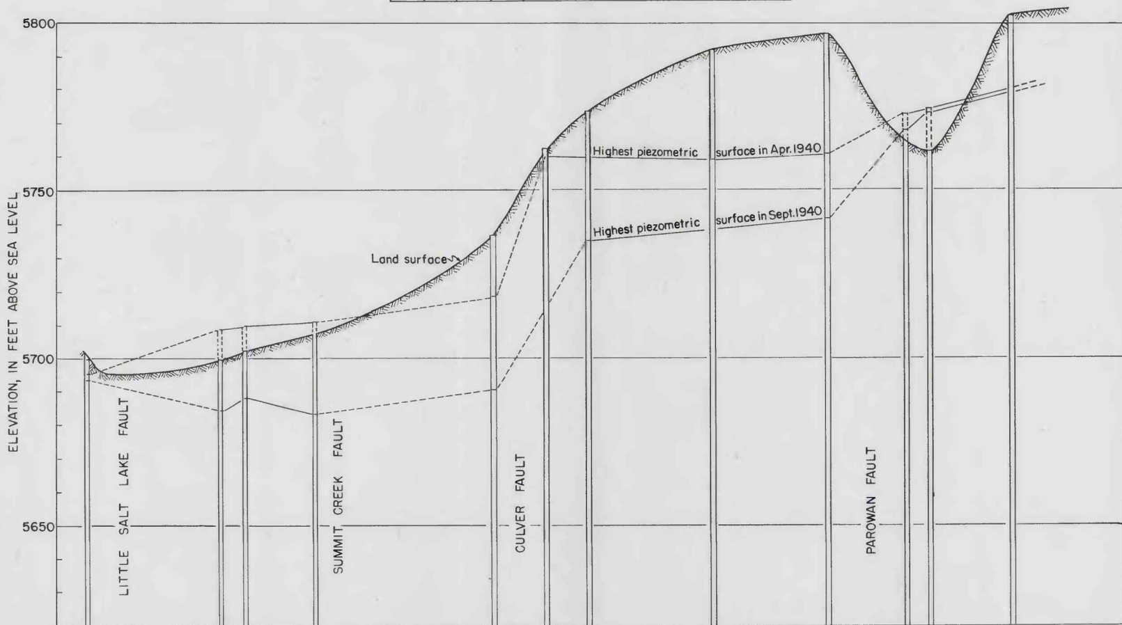
PROFILE ALONG THE SOUTH BOUNDARY OF T. 33 S. SHOWING POSITION OF THE HIGHEST PIEZOMETRIC SURFACE IN APRIL AND SEPTEMBER 1940
