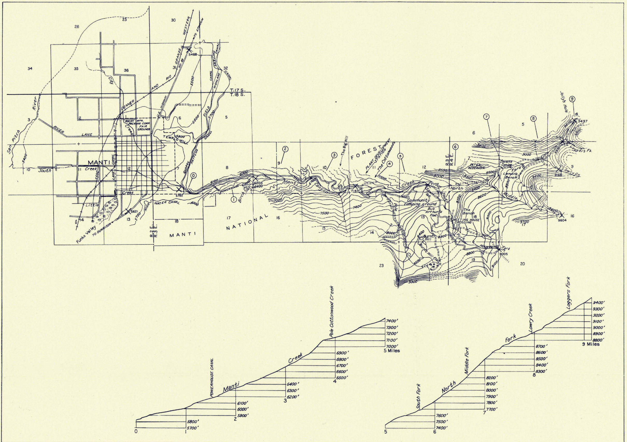
PLAN AND PROFILE OF MANTI CREEK, INCLUDING NORTH FORK, SANPETE COUNTY, UTAH
