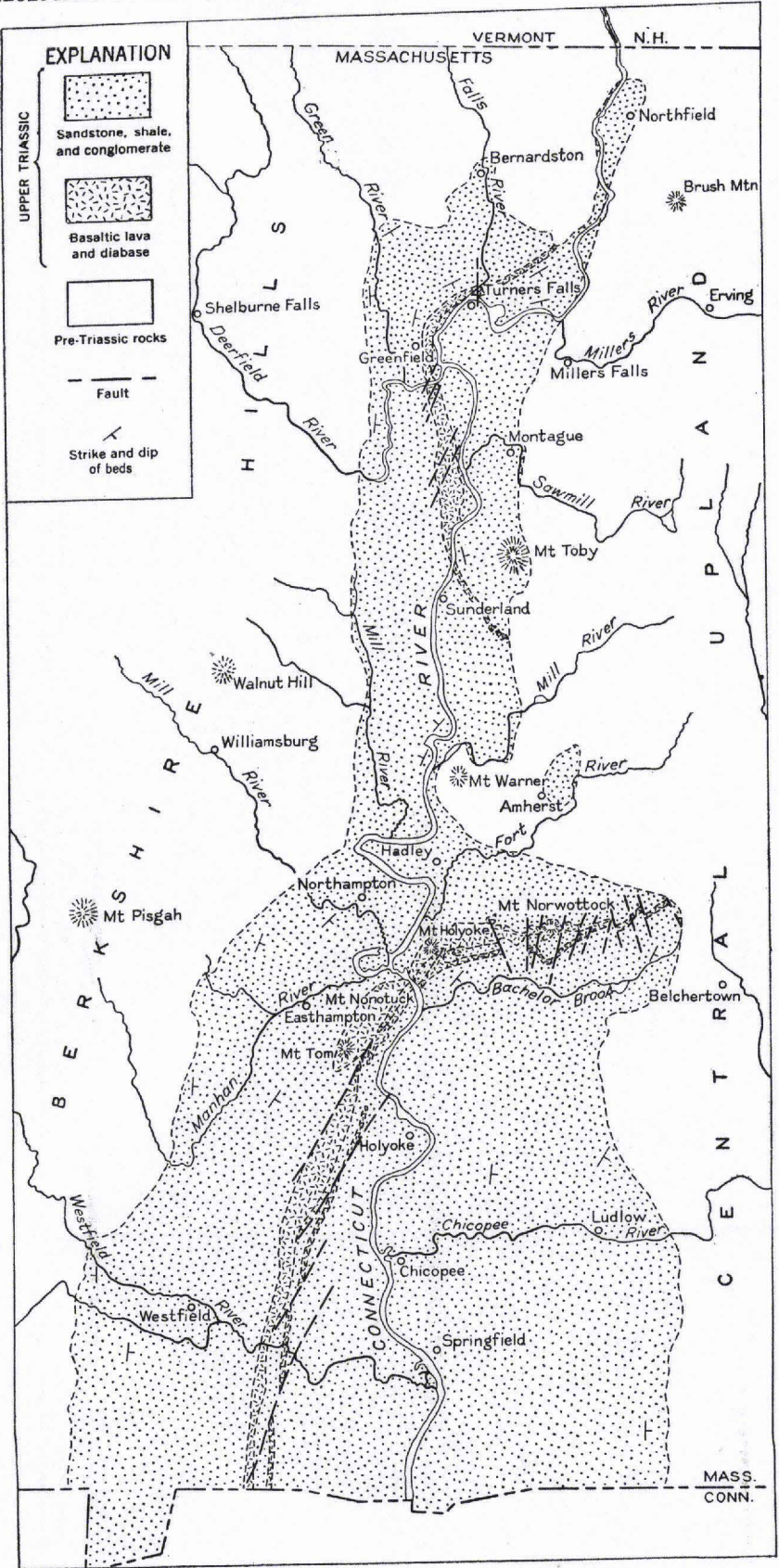
GENERAL GEOLOGIC MAP OF THE MASSACHUSETTS PART OF THE CONNECTICUT VALLEY AND ADJACENT AREA.
