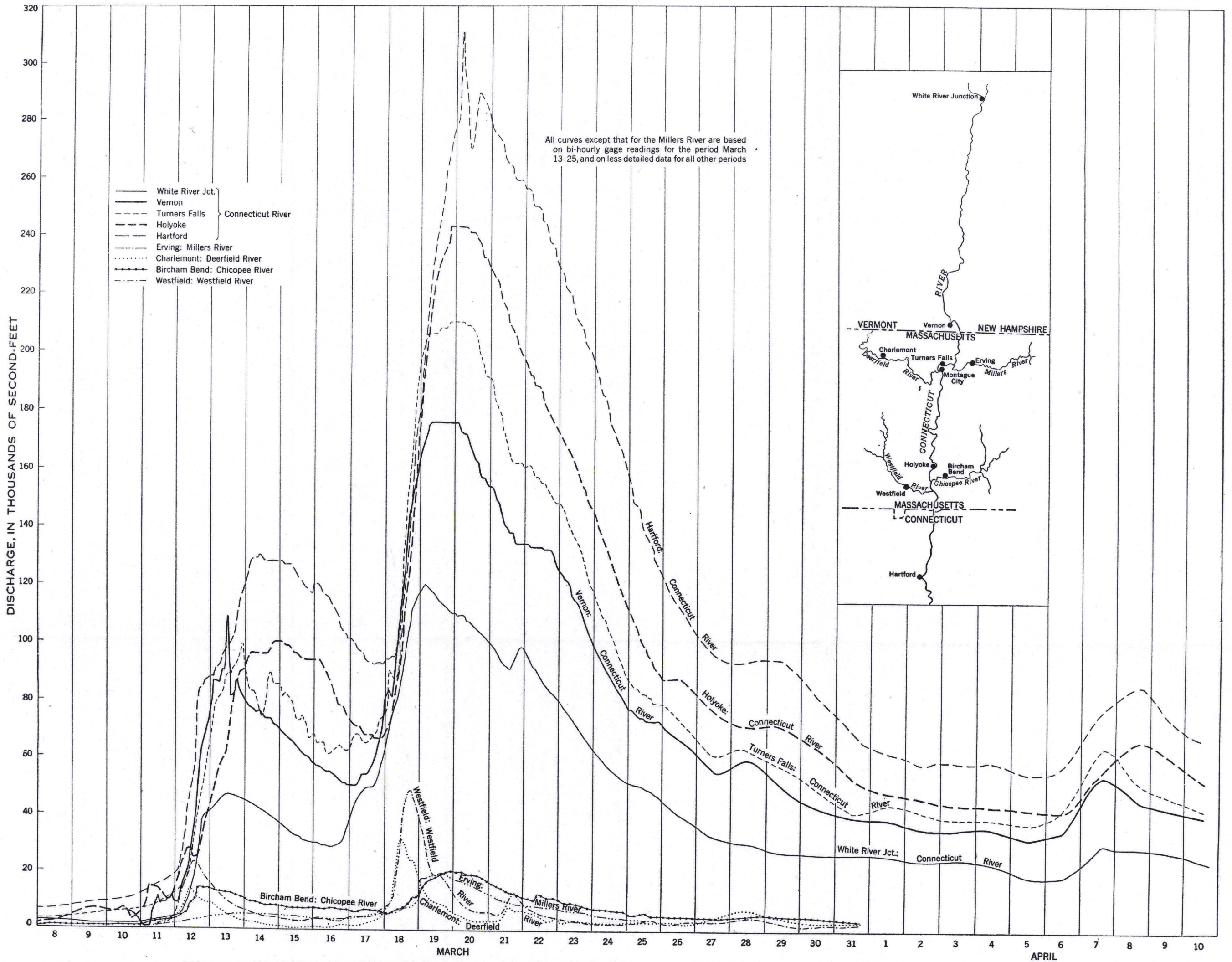
DISCHARGE CURVES FOR THE CONNECTICUT RIVER AND IMPORTANT TRIBUTARIES IN MASSACHUSETTS DURING THE PERIOD MARCH 8 TO APRIL 10, 1936.
