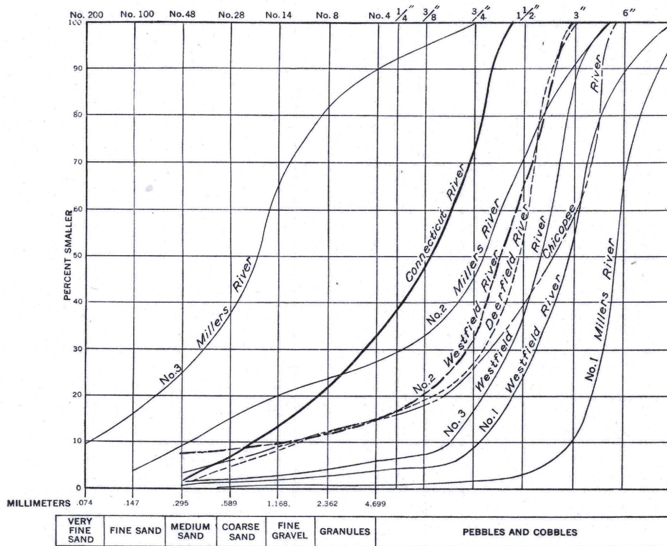
A. Sieve analyses for Connecticut, Westfield, Millers, and Deerfield Rivers
