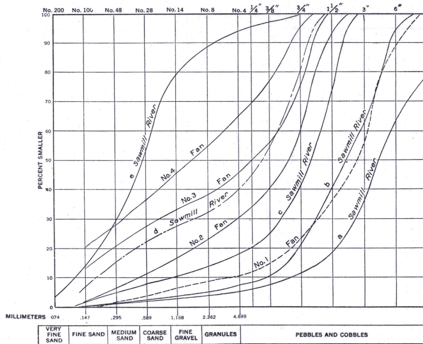
B. Sieve analyses for Sawmill River and for small debris fan west of Montague
