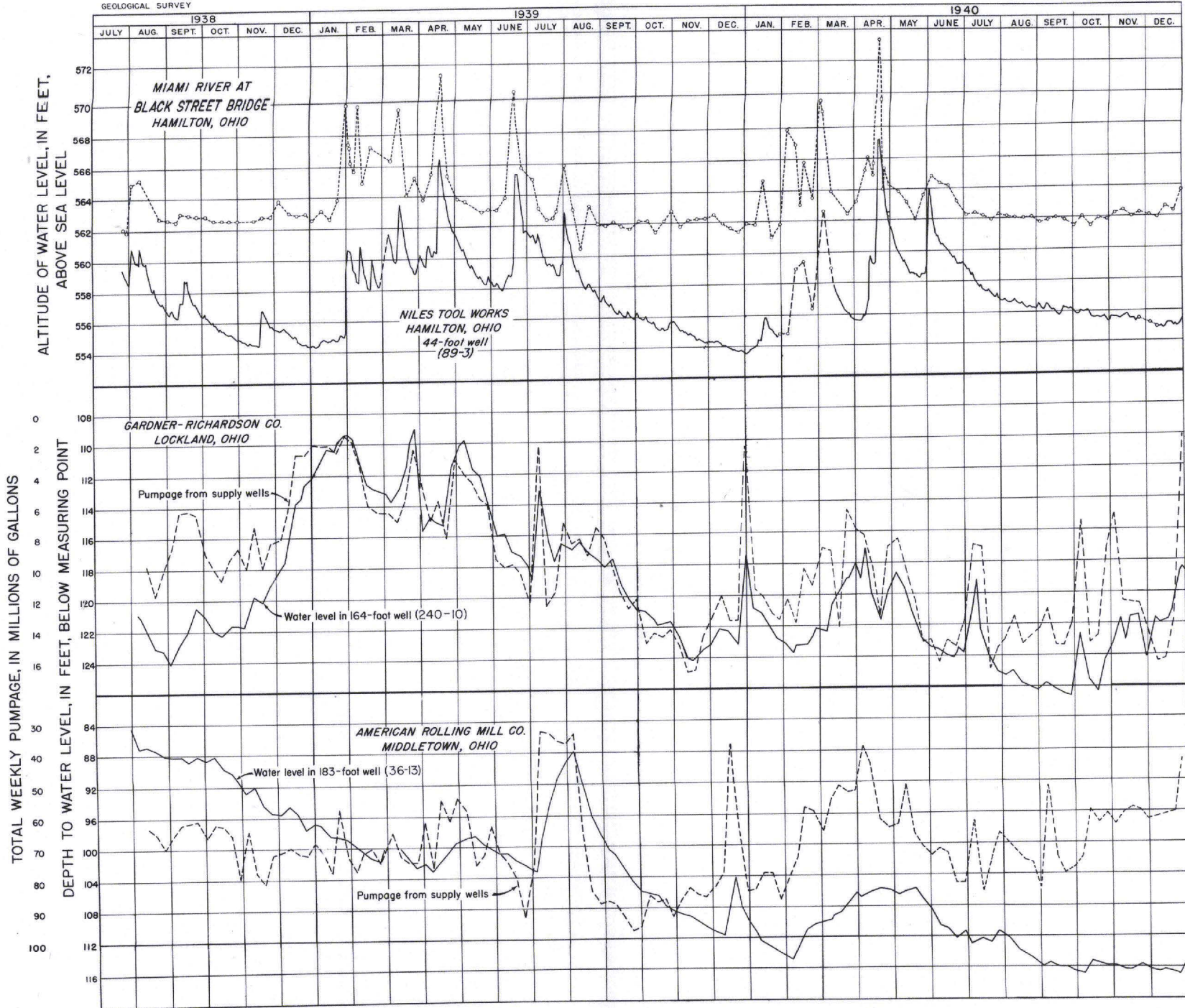
GRAPHS SHOWING RELATION OF WATER LEVELS IN OBSERVATION WELLS, SUPPLY WELLS, AND MIAMI RIVER
