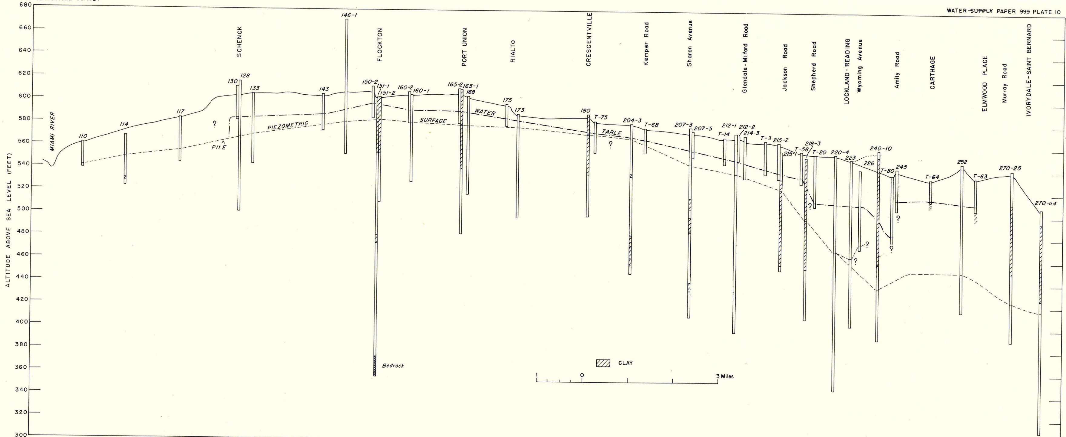
PROFILE OF LAND SURFACE, WATER TABLE, AND PIEZOMETRIC SURFACE IN THE MIAMI AND MILL CREEK VALLEYS FROM MIAMI RIVER SOUTH OF HAMILTON TO IVORYDALE, NOVEMBER 7-9, 1940
