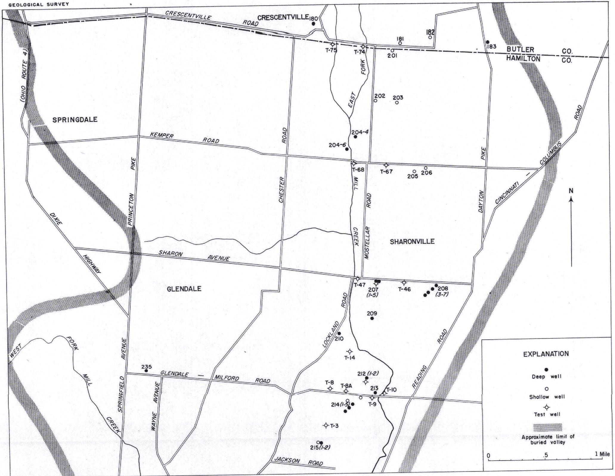
MAP OF MILL CREEK VALLEY FROM CRESCENTVILLE TO JACKSON ROAD, SHOWING LOCATION OF WELLS AND APPROXIMATE LIMITS OF BURIED VALLEY
