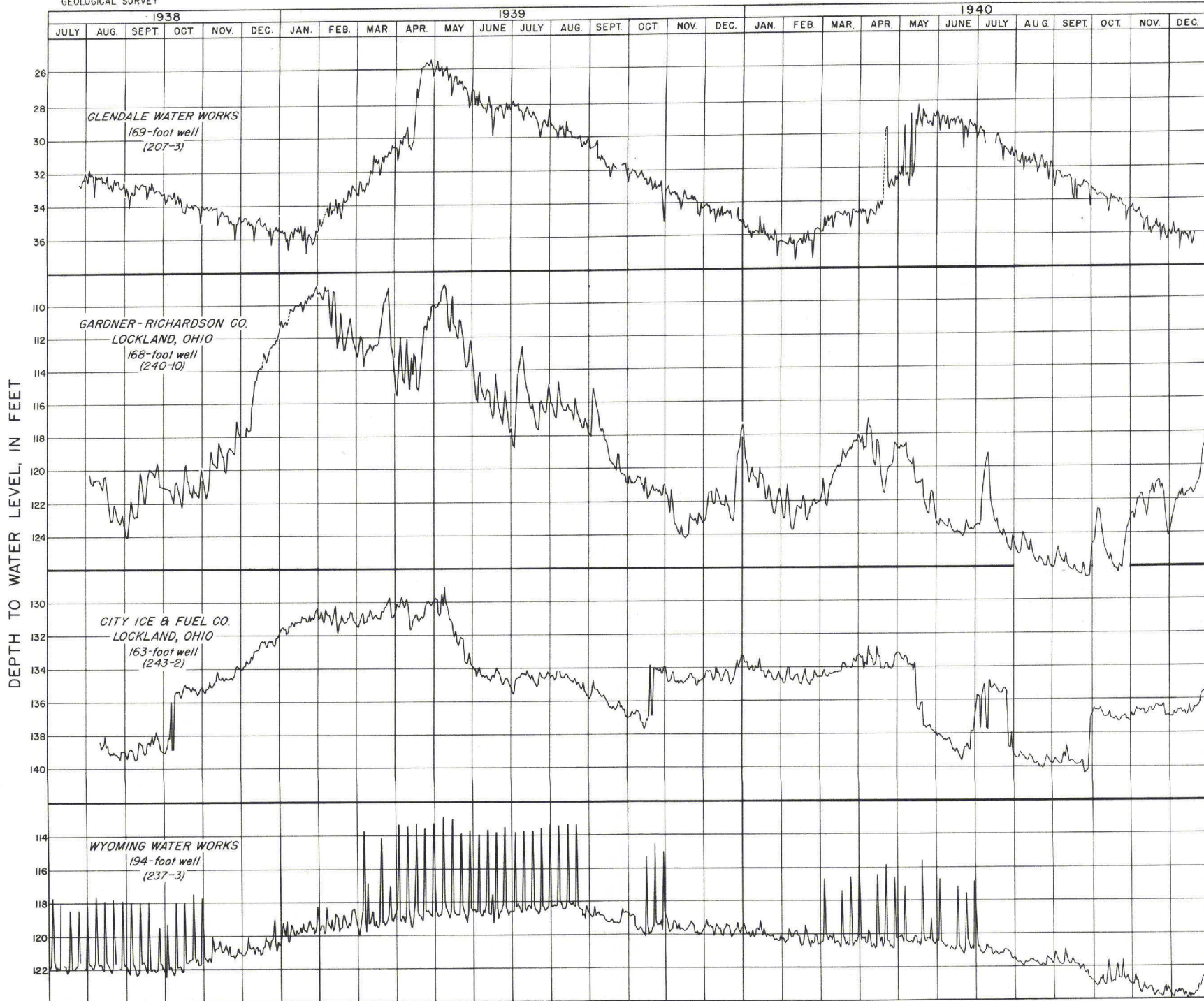
GRAPHS SHOWING LOWEST WATER LEVEL REACHED IN FOUR WELLS IN HAMILTON COUNTY, AS DETERMINED FROM RECORDER CHARTS, JULY 1, 1938, TO DECEMBER 31, 1940
