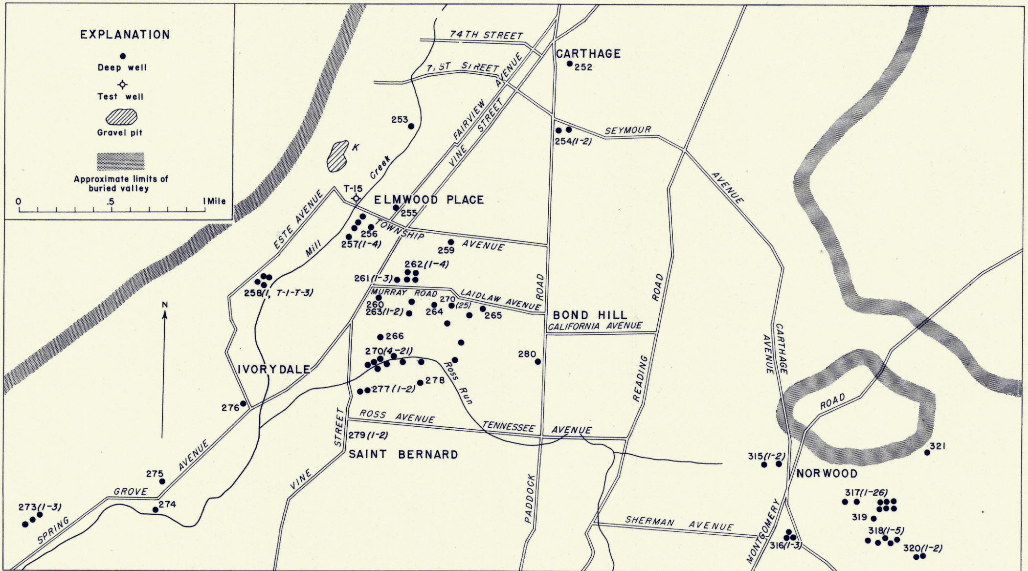
MAP OF IVORYDALE-SAINTE BERNARD AREA AND NORWOOD TROUGH SHOWING LOCATION OF WELLS AND APPROXIMATE LIMITS OF BURIED VALLEYS
