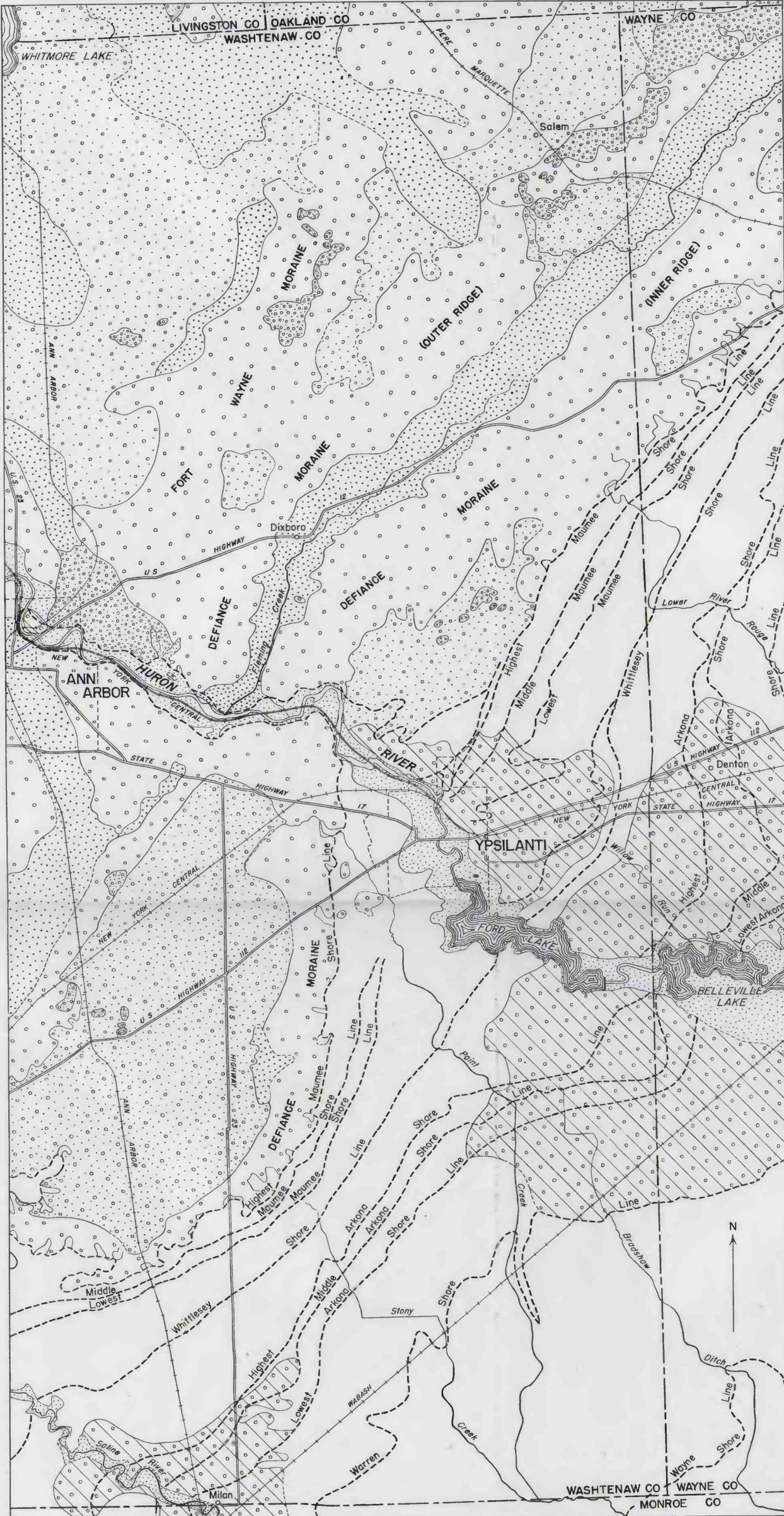
MAP SHOWING SURFACE FORMATIONS AND SHORE LINES OF GLACIAL LAKES IN THE YPSILANTI-ANN ARBOR AREA, MICHIGAN
