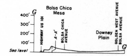
LAND-SURFACE PROFILES ALONG AND ACROSS THE NEWPORT-INGLEWOOD BELT, LONG BEACH-SANTA ANA AREA, CALIFORNIA
