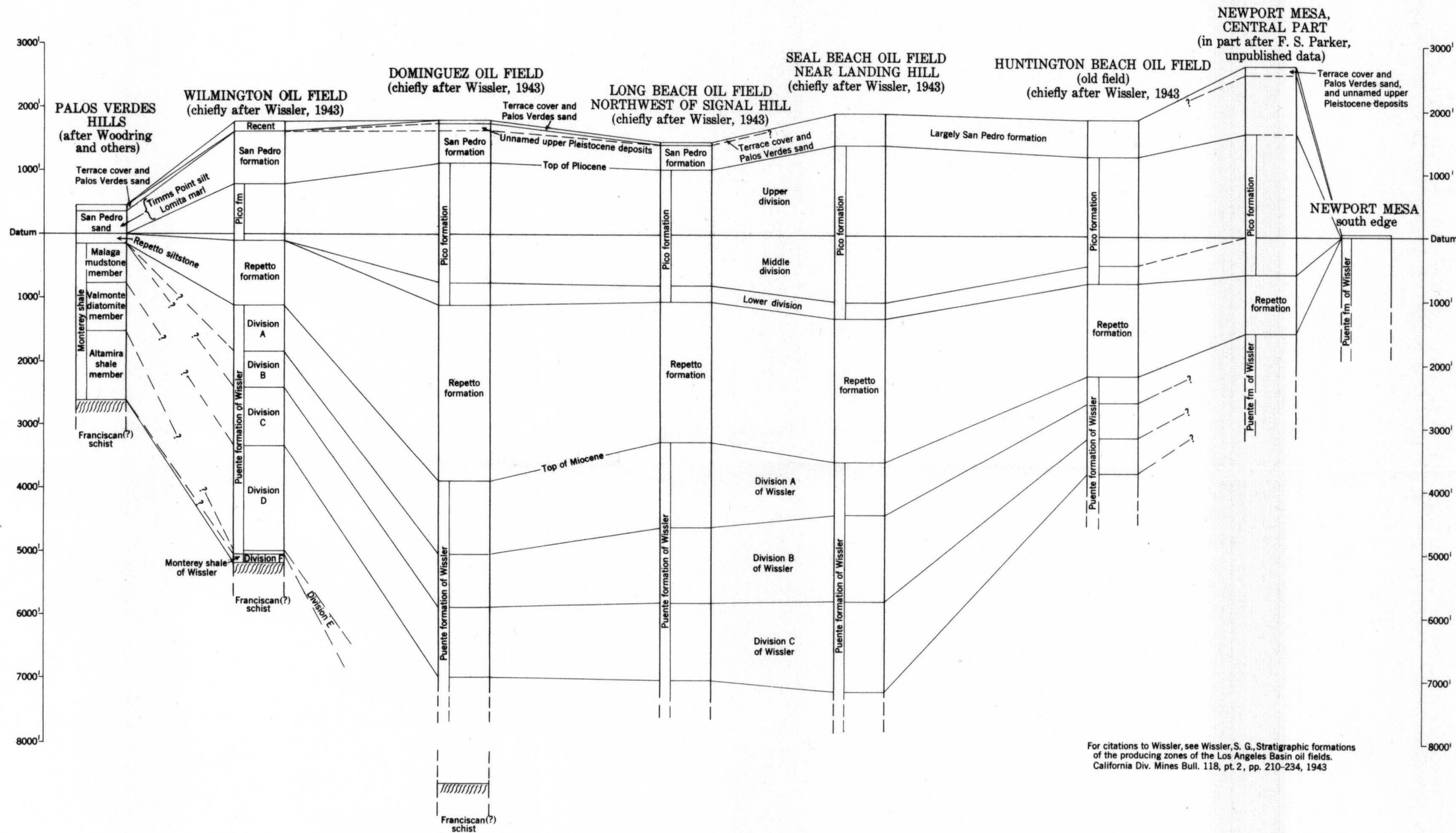
DIAGRAMMATIC CORRELATION OF STRATIGRAPHIC COLUMNS ALONG THE COASTAL ZONE OF THE LONG BEACH-SANTA ANA AREA, CALIFORNIA
