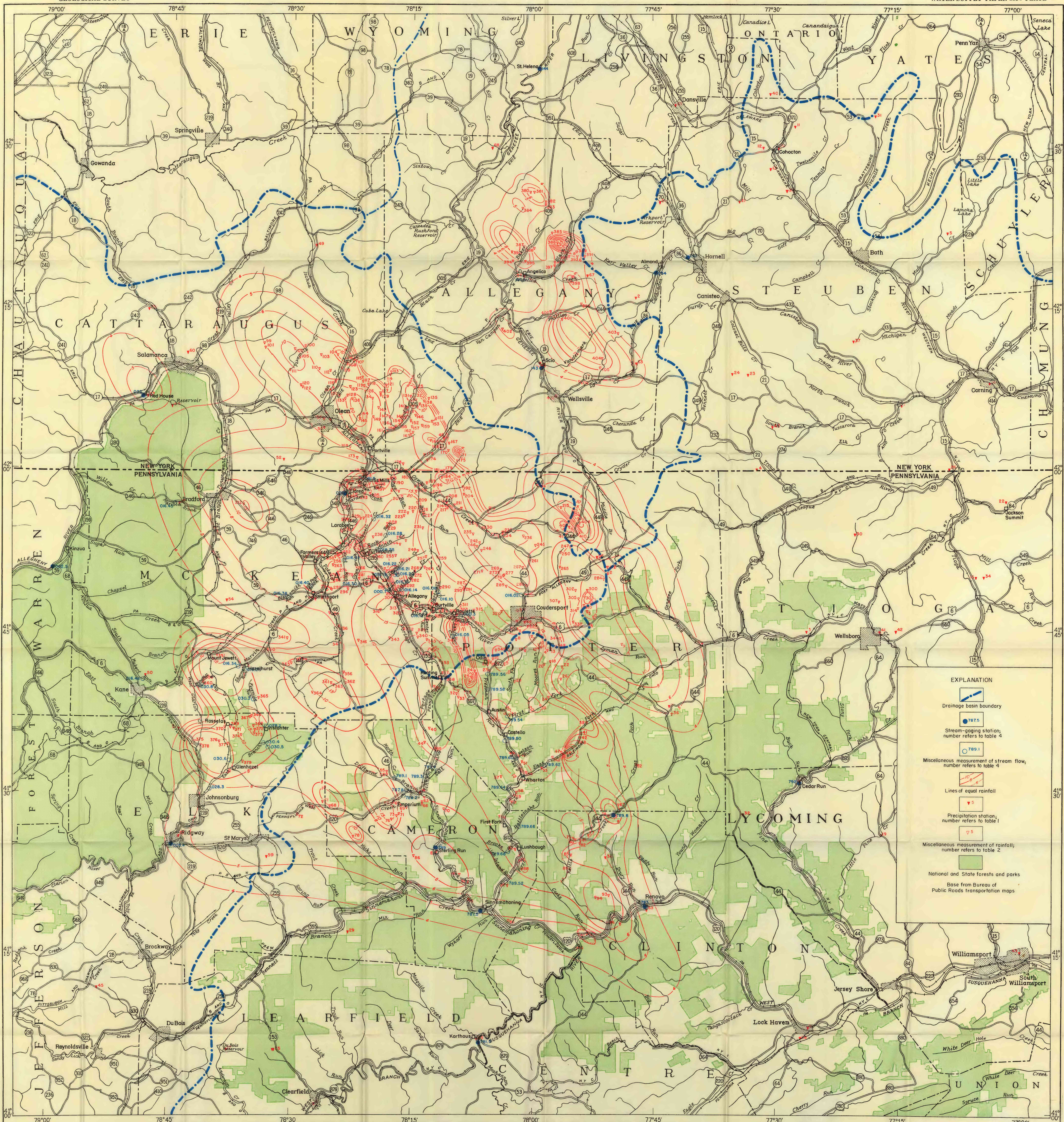
MAP OF FLOOD AREA SHOWING LOCATIONS OF STREAM-GAGING STATIONS, RAINFALL-MEASUREMENT POINTS, AND ISOHYETAL LINES FOR JULY 17-18, 1942
