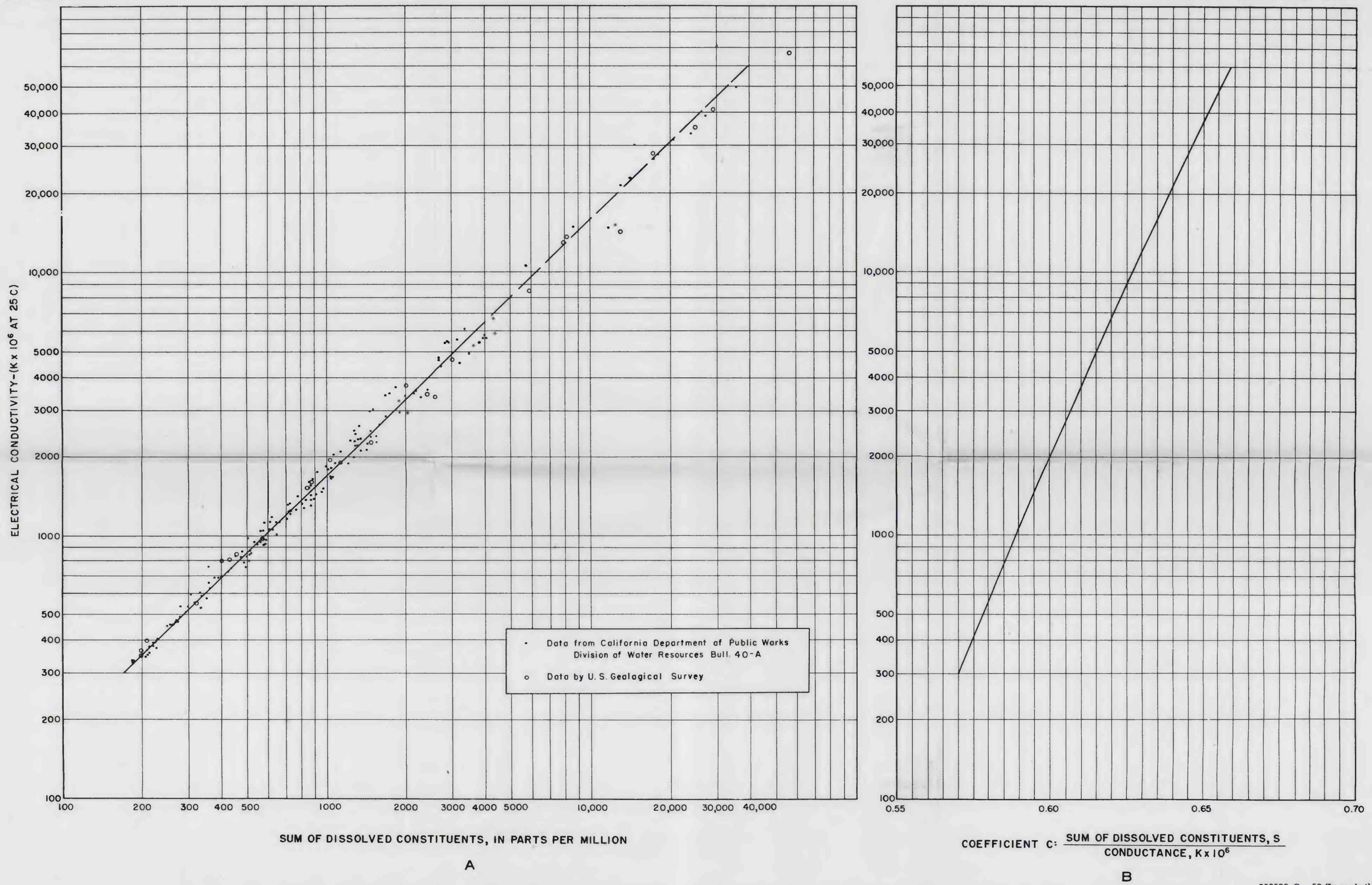
A. RELATION BETWEEN CONDUCTANCE AND SUM OF DISSOLVED CONSTITUENTS IN WATERS FROM 186 WELLS IN AND NEAR THE LONG BEACH-SANTA ANA AREA. B. RELATION BETWEEN CONDUCTANCE AND COEFFICIENT "C"
