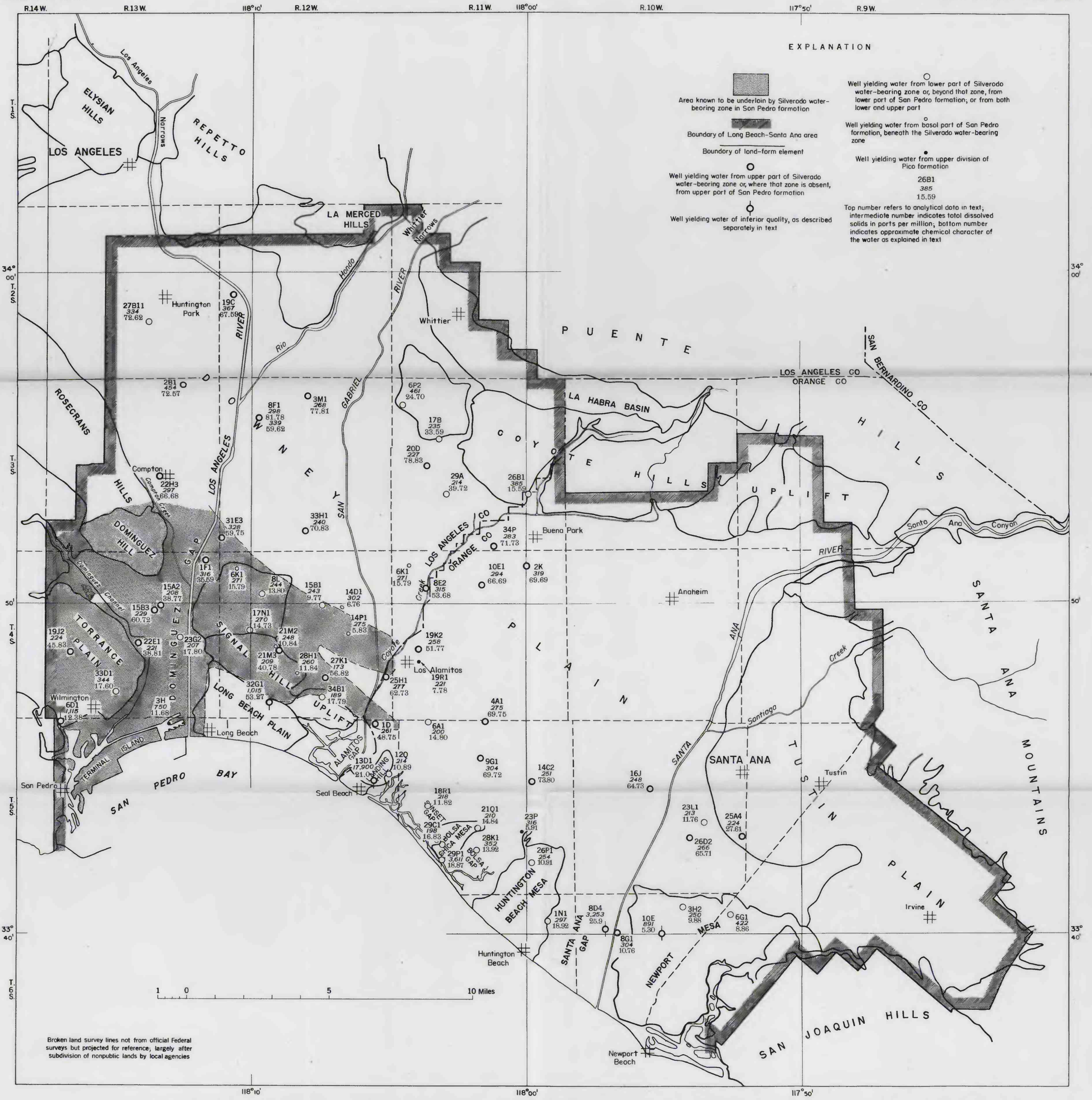
MAP OF THE LONG BEACH-SANTA ANA AREA SHOWING SOURCES OF REPRESENTATIVE NATIVE WATER FROM THE SILVERADO WATER-BEARING ZONE OF LOS ANGELES COUNTY, FROM SAN PEDRO FORMATION BEYOND THE EXTENT OF THAT ZONE, AND FROM THE UPPER DIVISION OF THE PICO FORMATION
