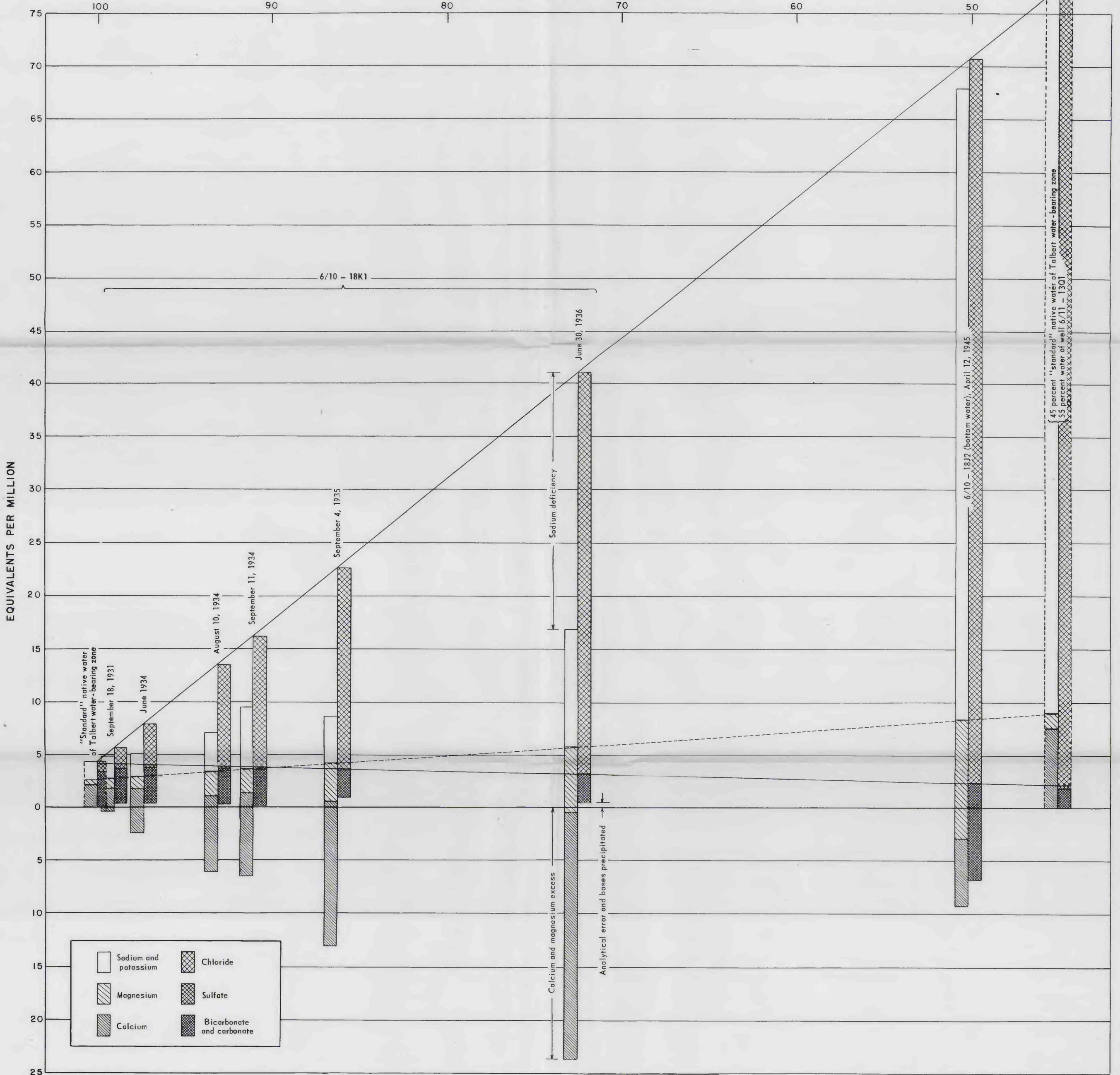
PROGRESSIVELY CONTAMINATED WATER FROM WELL 6/10-18K1 (NEWPORT BEACH, WELL 4), IN RELATION TO HYPOTHETICAL MIXTURE OF "STANDARD" NATIVE WATER FROM THAT WELL WITH BRINE FROM WELL 6/11-13Q1, ALSO IN RELATION TO BOTTOM WATER FROM WELL 6/10-18J2
