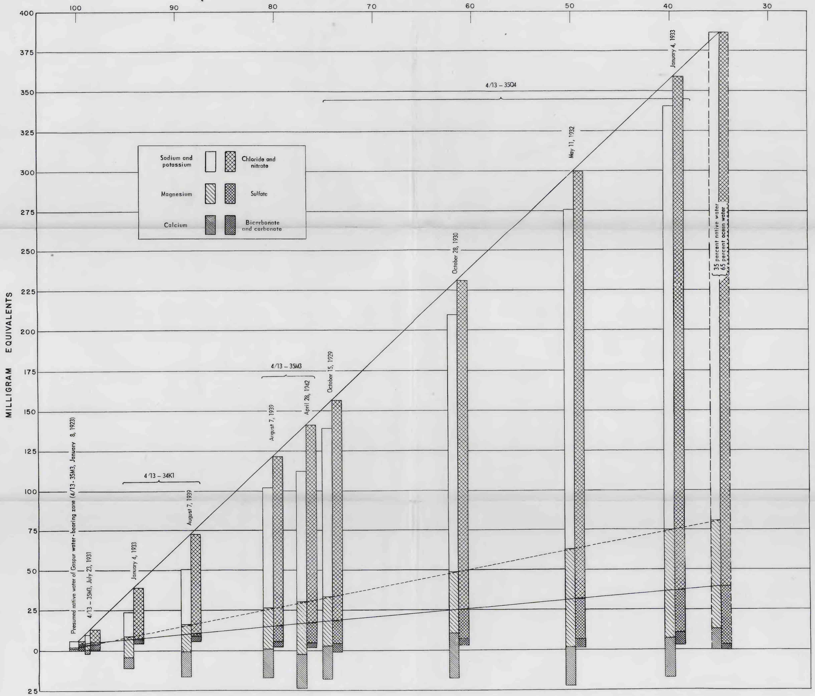
PROGRESSIVELY CONTAMINATED WATERS FROM WELLS TAPPING THE GASPUR WATER-BEARING ZONE NEAR THE COAST. IN RELATION TO HYPOTHETICAL MIXTURE OF THE PRESUMED NATIVE WATER FROM THAT ZONE WITH OCEAN WATER
