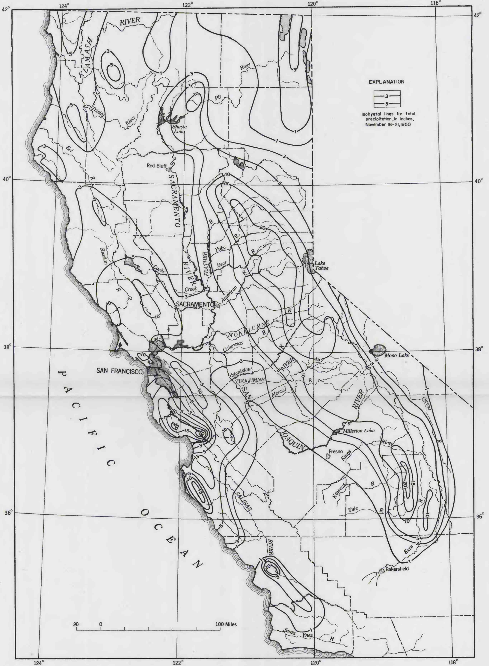
ISOHYETAL MAP FOR STORM OF NOVEMBER 16-21, 1950, CENTRAL VALLEY BASIN, CALIFORNIA
