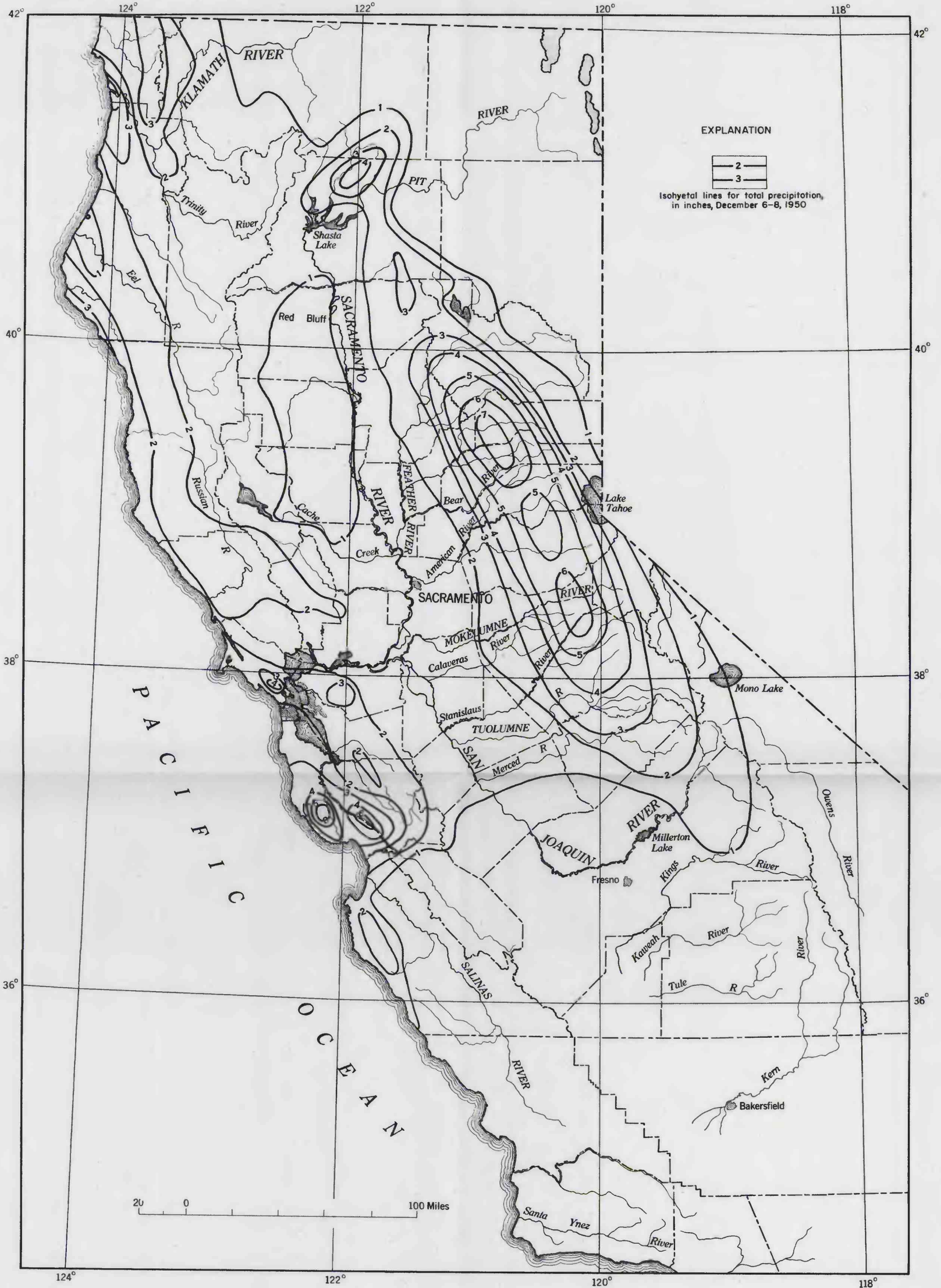
ISOHYETAL MAP FOR STORM OF DECEMBER 6-8, 1950, CENTRAL VALLEY BASIN, CALIFORNIA
