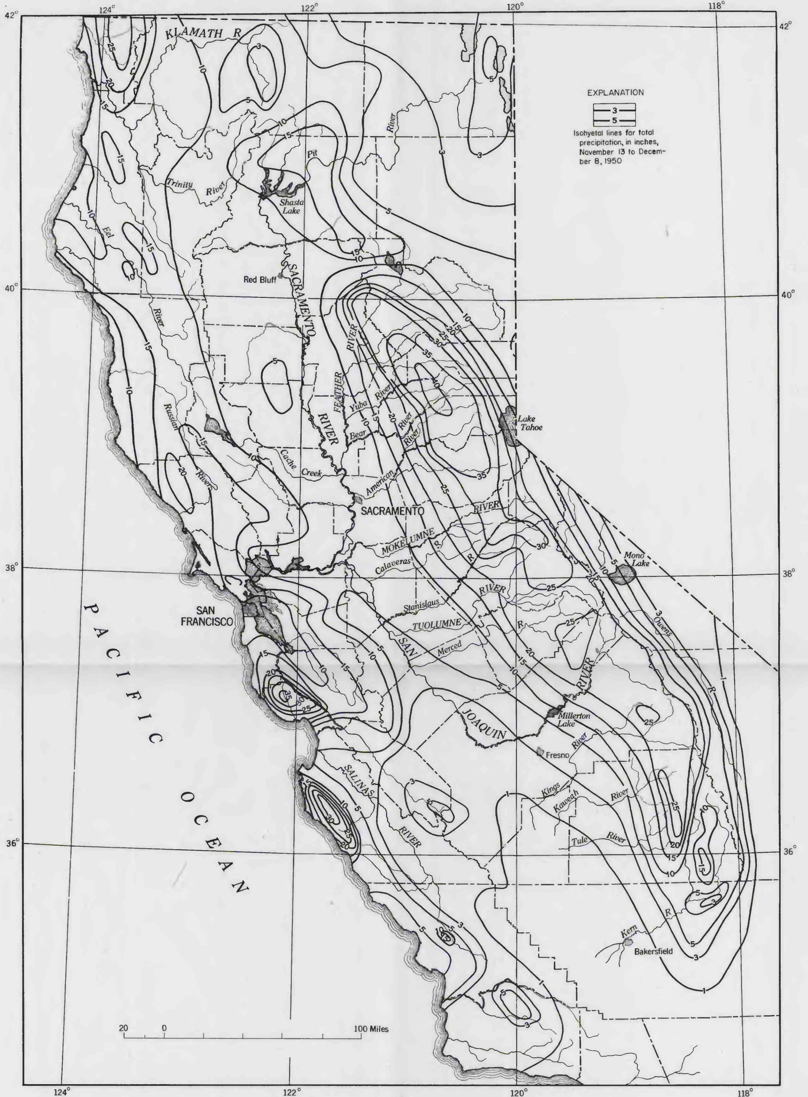
ISOHYETAL MAP SHOWING TOTAL PRECIPITATION DURING PERIOD NOVEMBER 13 TO DECEMBER 8, 1950, CENTRAL VALLEY BASIN, CALIFORNIA
