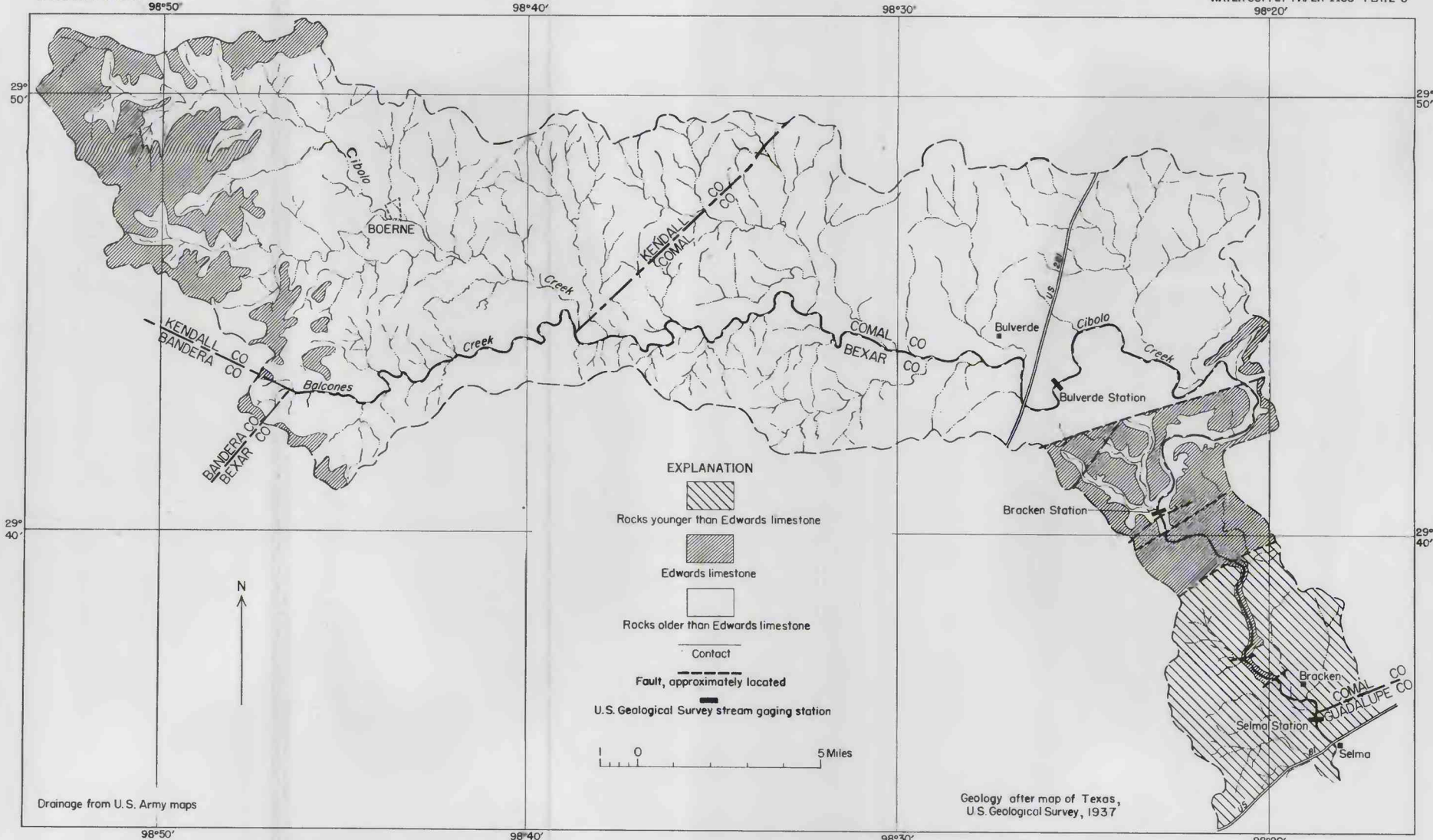
MAP OF CIBOLO CREEK BASIN SHOWING GEOLOGY AND STREAM GAGING STATIONS
