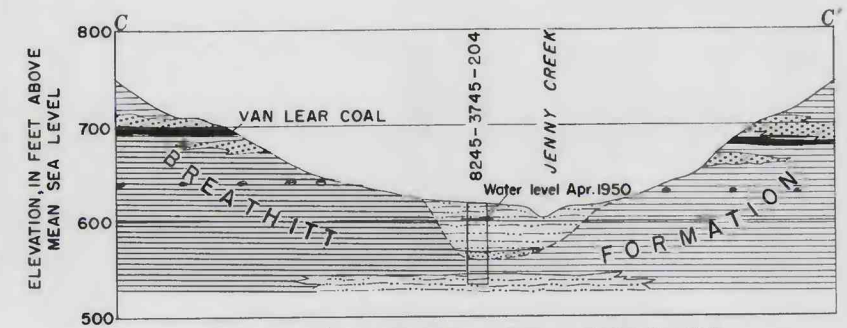
SECTION C-C' ACROSS JENNY CREEK NEAR COLLISTA
