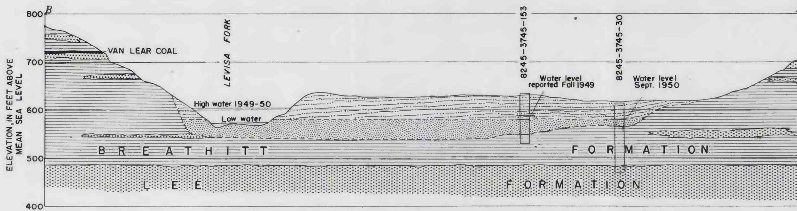
SECTION B-B' ACROSS LEVISA FORK NEAR PAINTSVILLE
