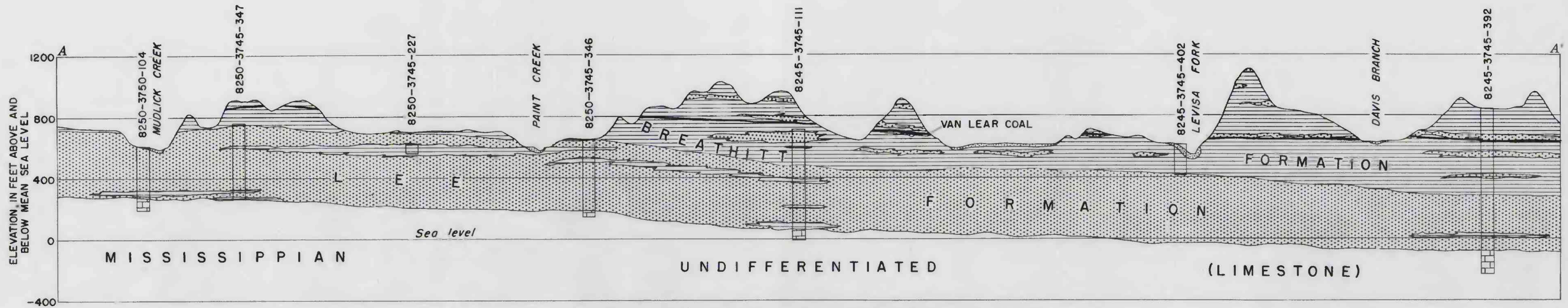
SECTION A-A' FROM MUDLICK CREEK SOUTHEAST TO DAVIS BRANCH
