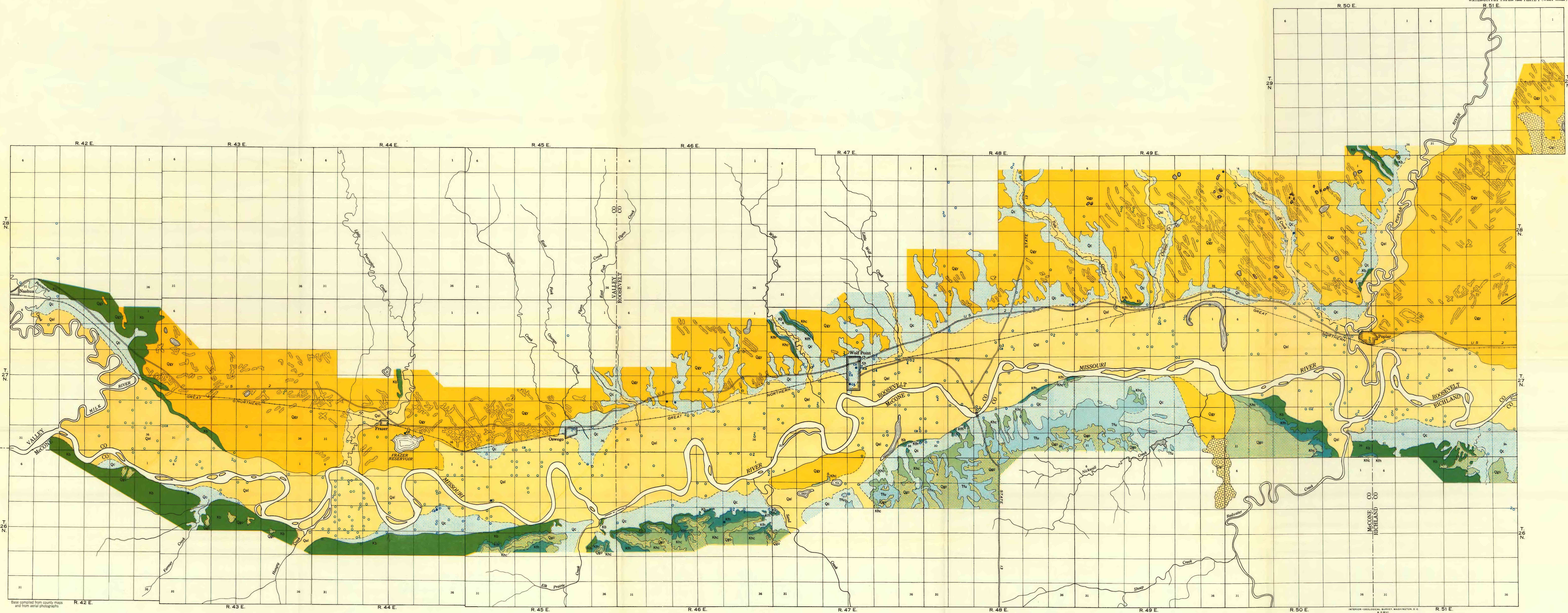
SURFICIAL GEOLOGY OF MISSOURI RIVER PUMPING UNITS, WITH LOCATIONS OF WELLS, MISSOURI-SOURIS IRRIGATION PROJECT, MONTANA
