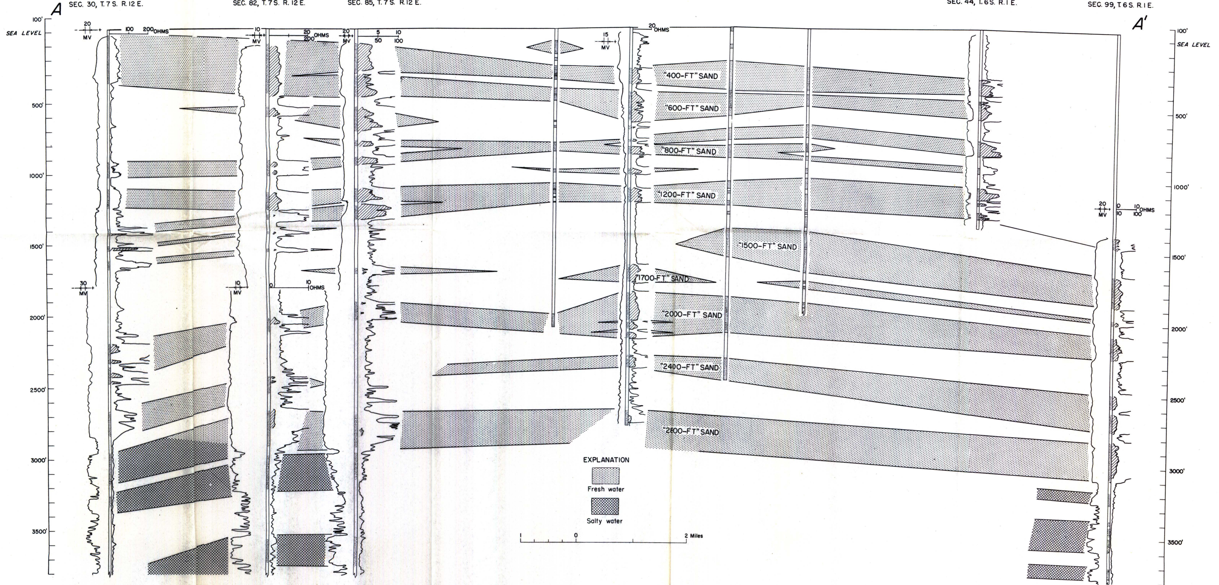
GEOLOGIC CROSS SECTION THROUGH BATON ROUGE ALONG LINE A-A' AS SHOWN ON FIGURE 5
