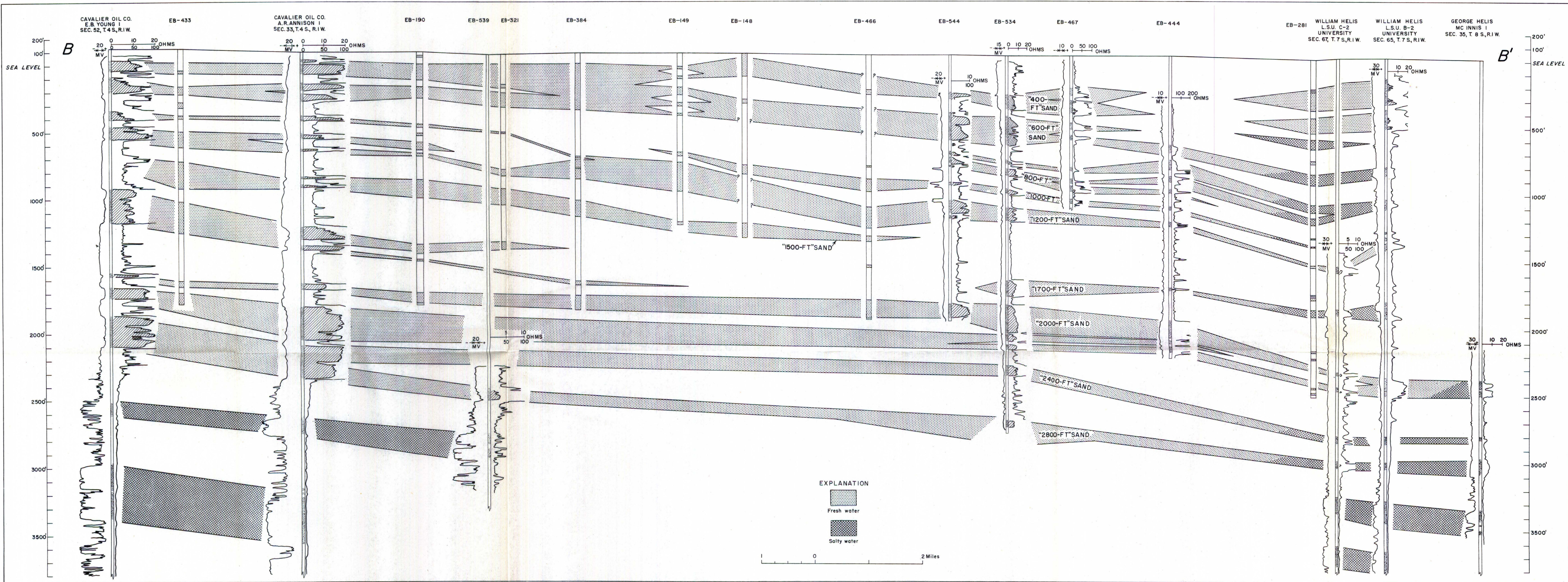
GEOLOGIC CROSS SECTION THROUGH BATON ROUGE ALONG LINE B-B' AS SHOWN ON FIGURE 5
