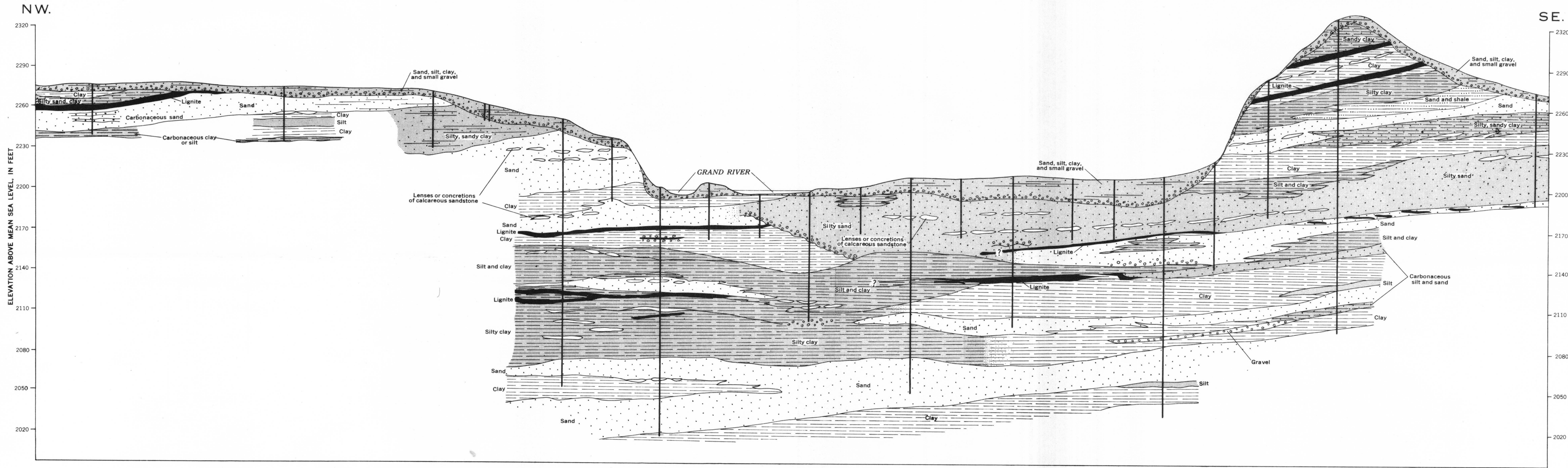
GEOLOGIC SECTION OF GRAND RIVER VALLEY AT SHADEHILL DAM SITE
