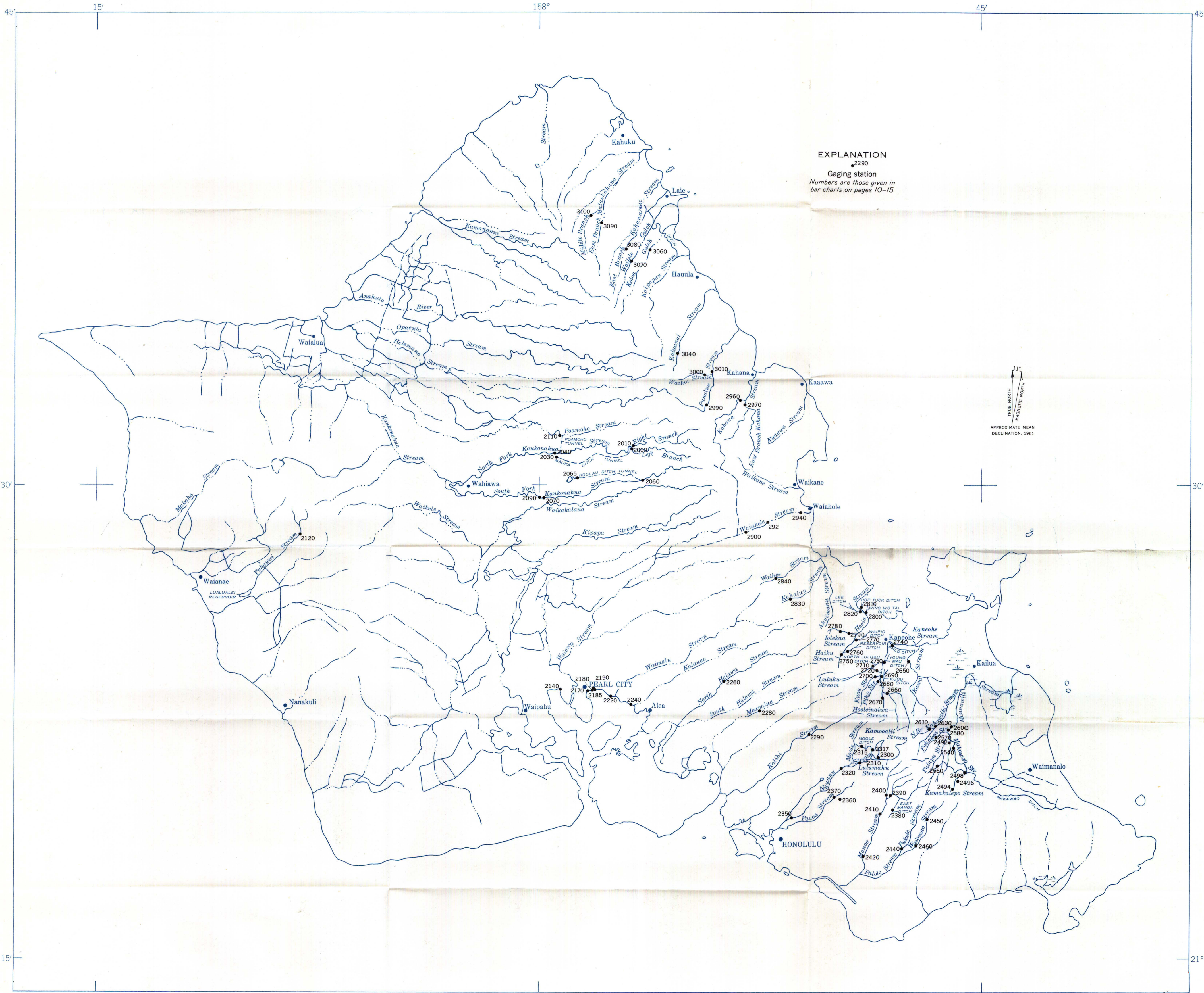
MAP OF OAHU SHOWING LOCATION OF GAGING STATIONS FOR WHICH RECORDS ARE INCLUDED IN THIS REPORT
