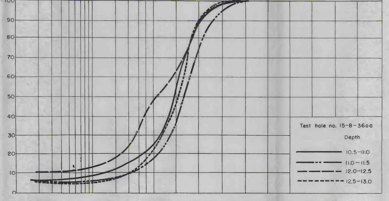
GRAPHS SHOWING RESULTS OF PARTICLE-SIZE ANALYSES OF SAMPLES OF THE MANTLE-ROCK FROM TEST HOLES IN THE PRAIRIE CREEK UNIT, MERRICK COUNTY, NEBRASKA
