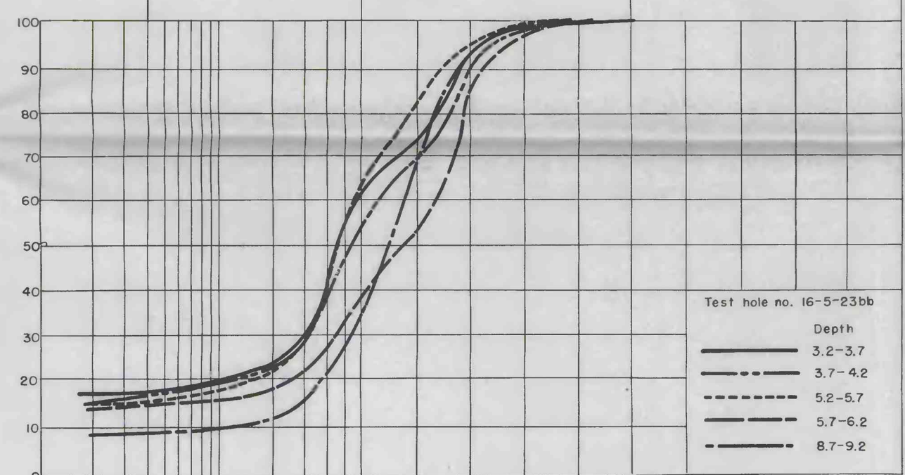
GRAPHS SHOWING RESULTS OF PARTICLE-SIZE ANALYSES OF SAMPLES OF THE MANTLE-ROCK FROM TEST HOLES IN THE PRAIRIE CREEK UNIT, NANCE COUNTY, NEBRASKA
