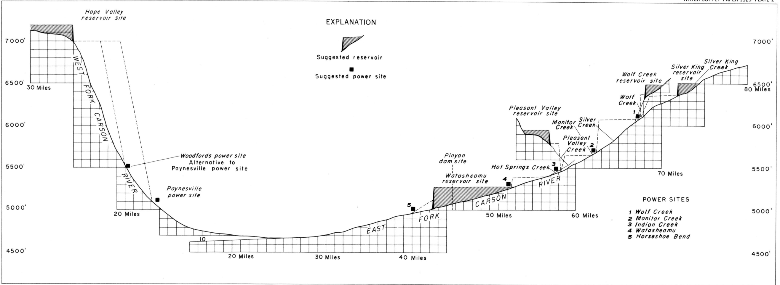
PROFILES OF EAST AND WEST FORK CARSON RIVER, SHOWING POWER AND STORAGE SITES, UPPER CARSON RIVER BASIN, CALIFORNIA
