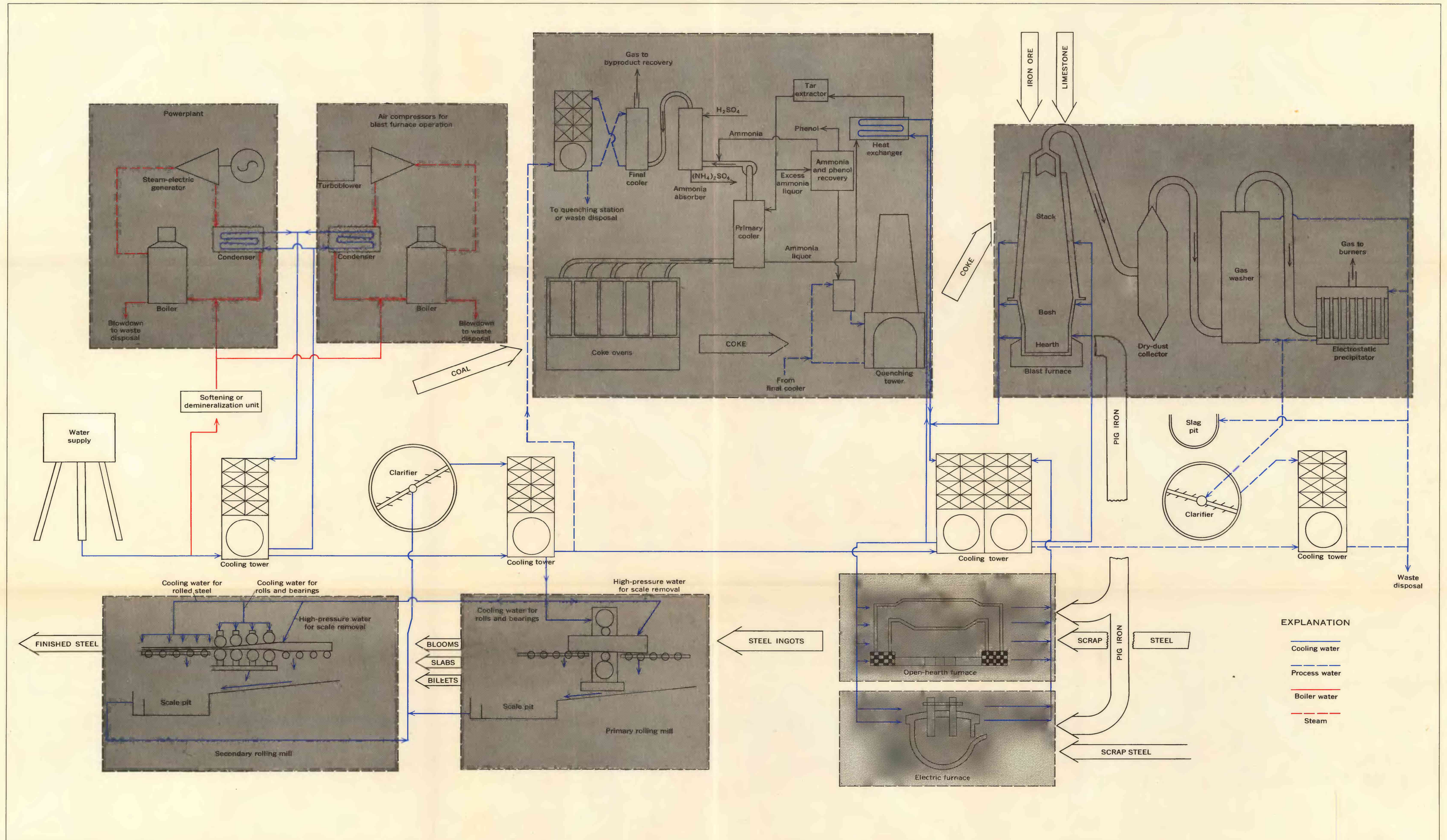
DIAGRAM SHOWING THE WATER SYSTEM OF A HYPOTHETICAL INTEGRATED STEEL PLANT
