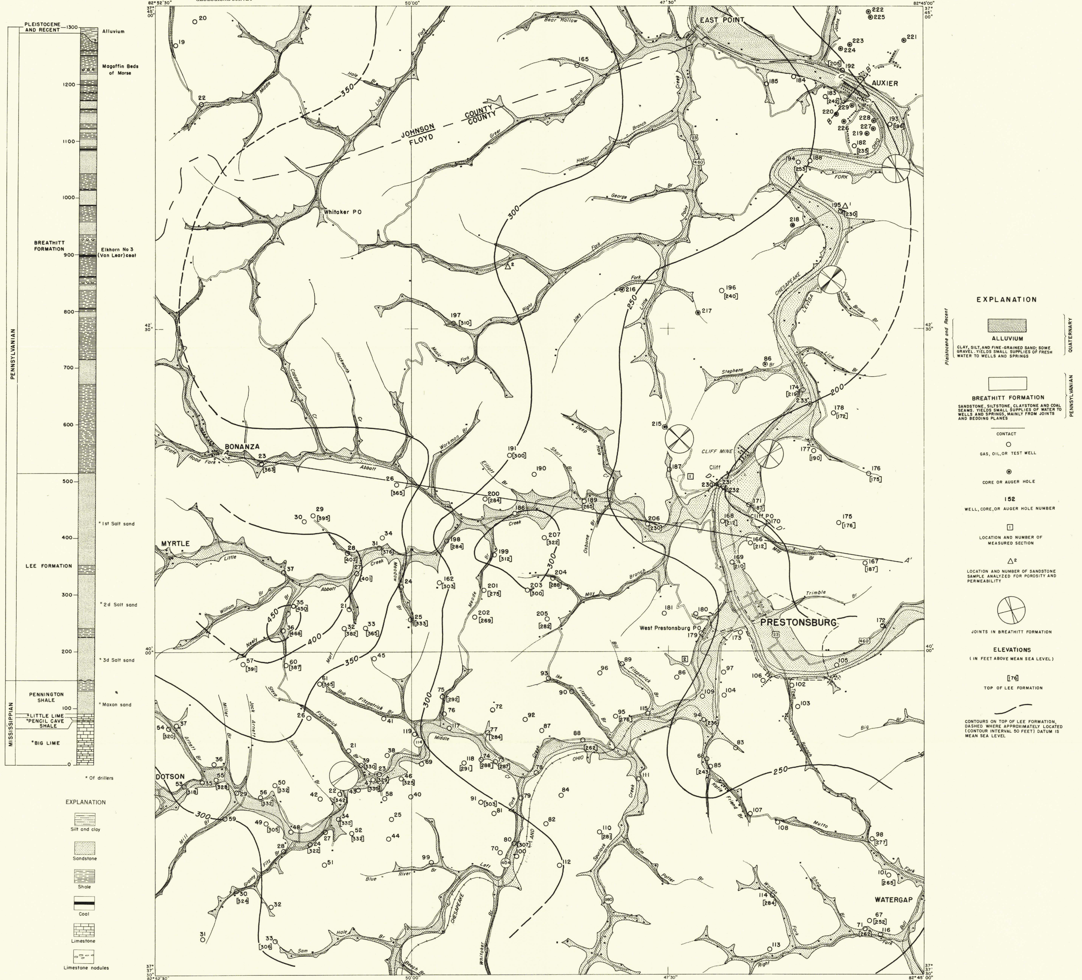
GEOLOGIC MAP OF PRESTONBURG QUADRANGLE, KENTUCKY, SHOWING CONTOURS ON TOP OF THE LEE FORMATION
