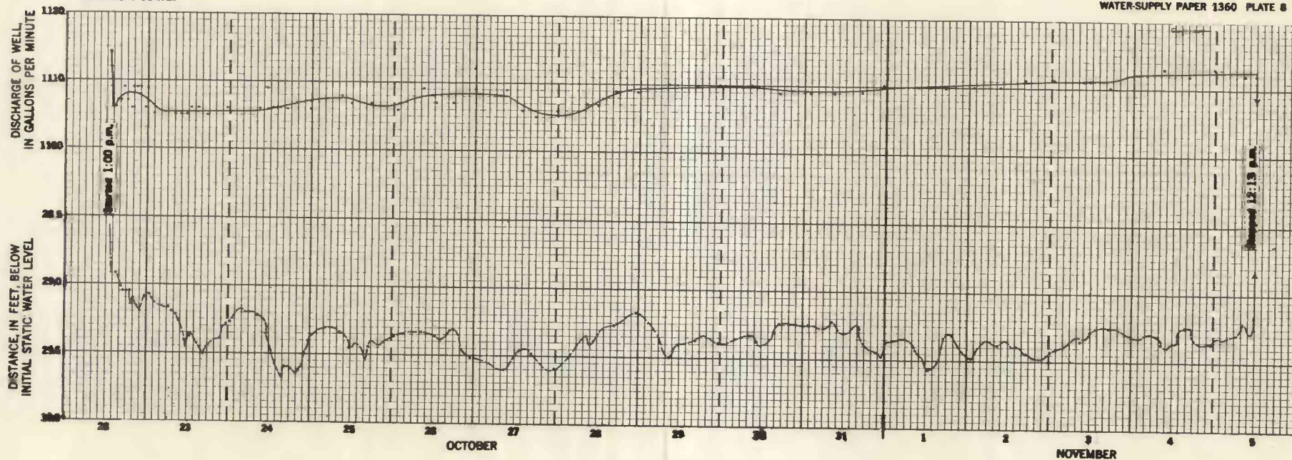
GRAPHS OF DISCHARGE AND WATER LEVEL IN PUMPED WELL, NORTHEASTERN SECTION OF LOUISVILLE AREA, 1946
