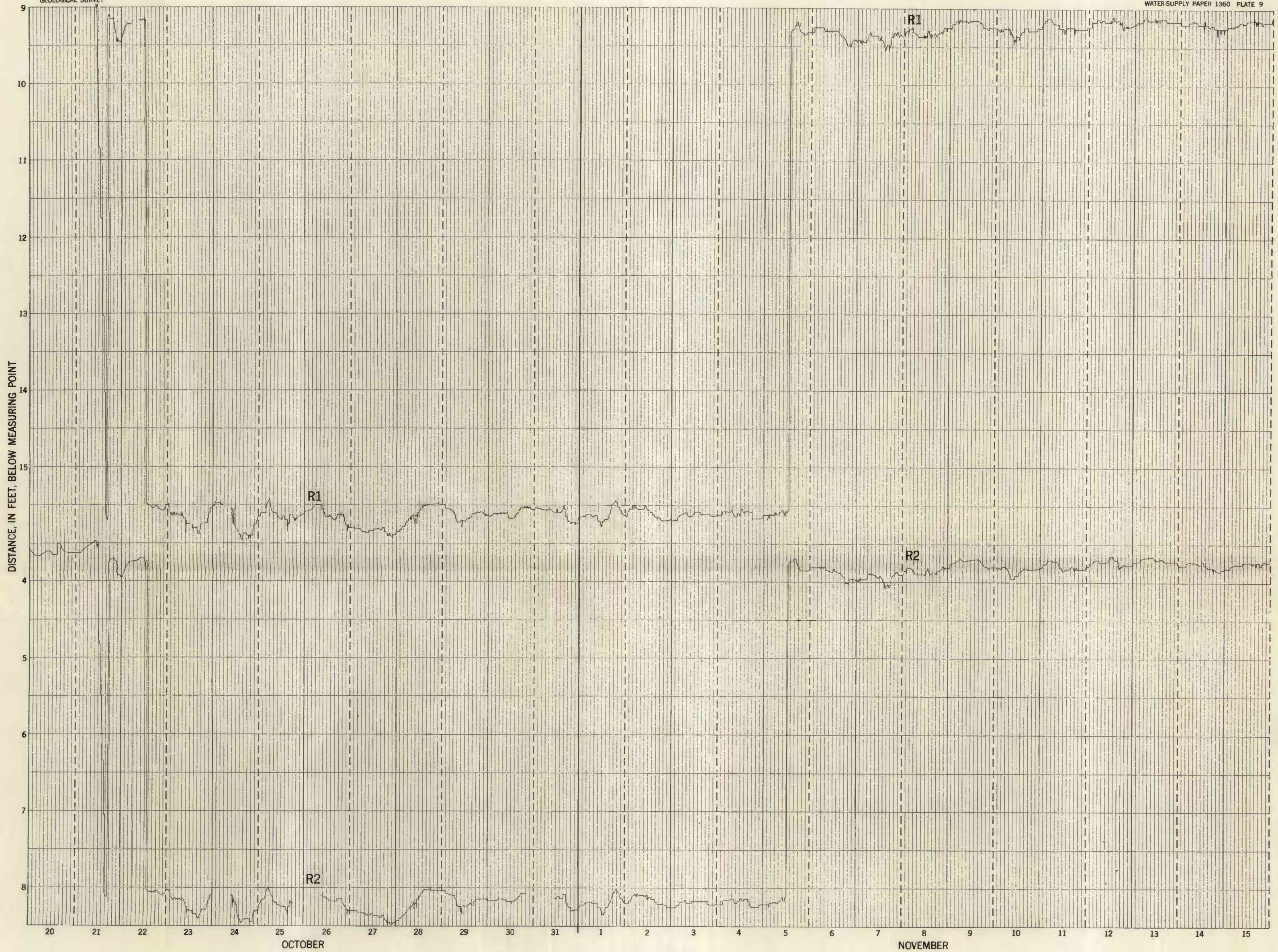
GRAPHS OF WATER LEVEL IN OBSERVATION WELLS R1 AND R2 DURING PUMPING TEST IN NORTHEASTERN SECTION OF LOUISVILLE AREA, 1946
