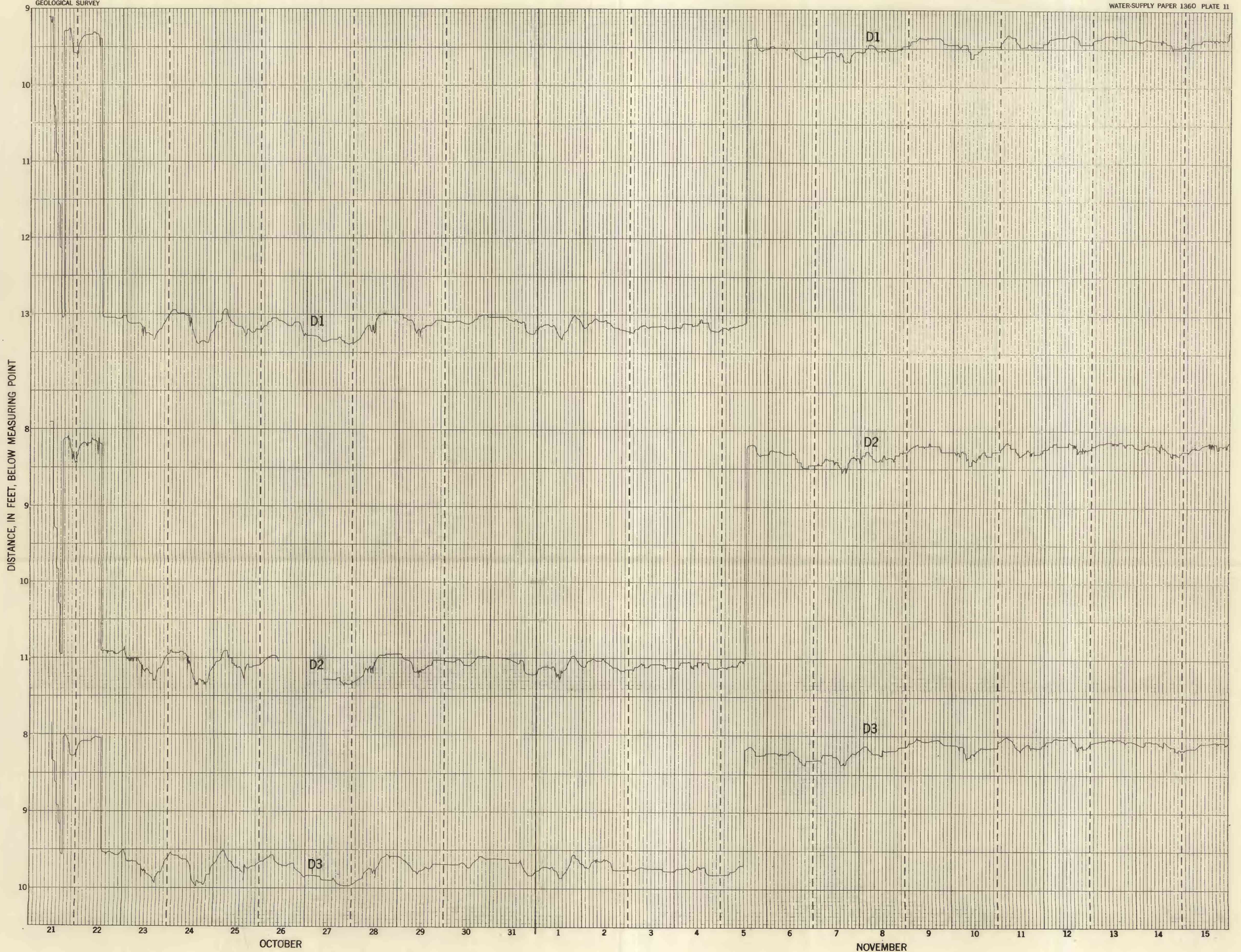
GRAPHS OF WATER LEVEL IN OBSERVATION WELLS D1, D2, AND D3 DURING PUMPING TEST IN NORTHEASTERN SECTION OF LOUISVILLE AREA, 1946
