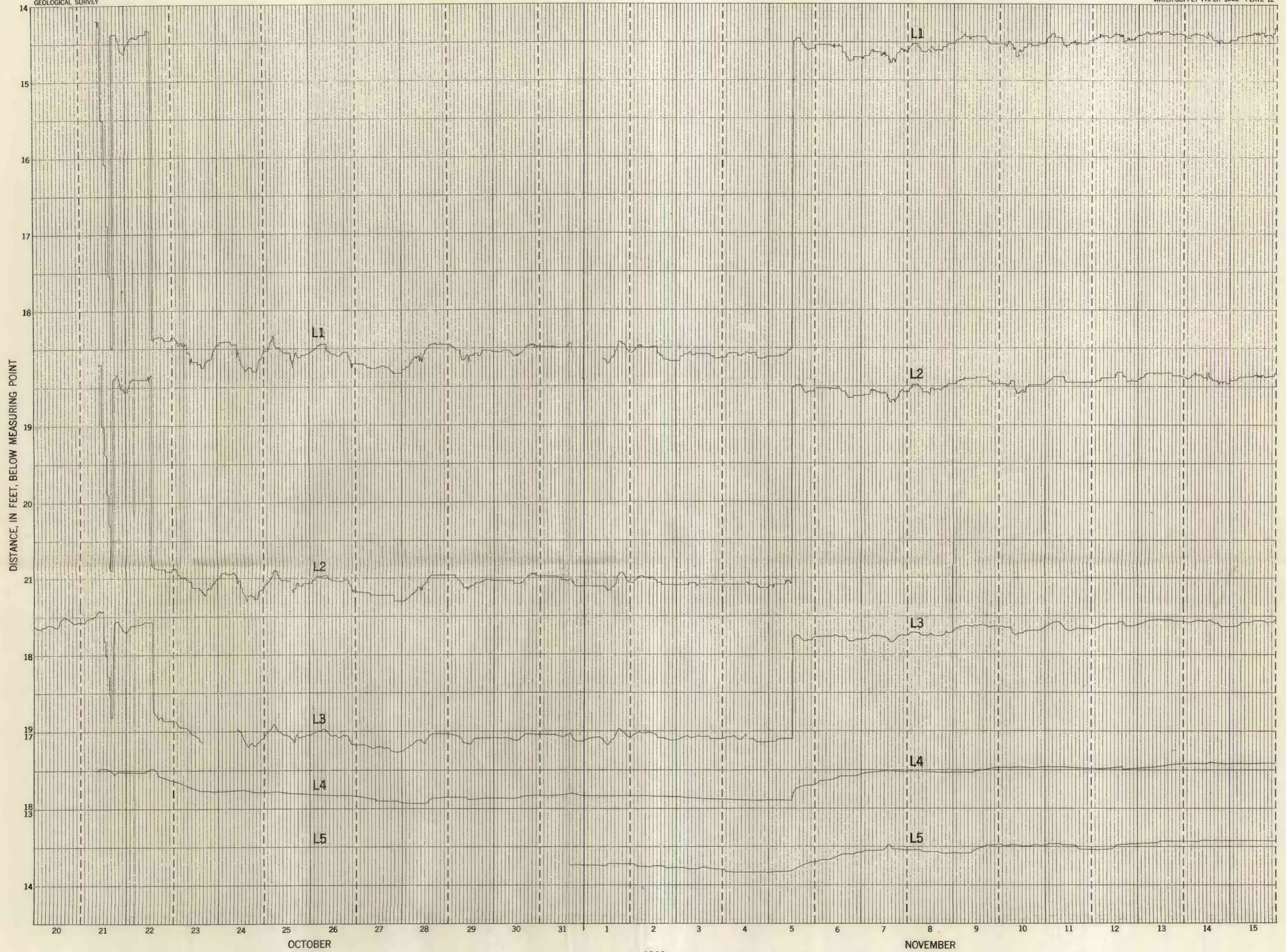
GRAPHS OF WATER LEVEL IN OBSERVATION WELLS L1-L5, INCLUSIVE, DURING PUMPING TEST IN NORTHEASTERN SECTION OF LOUISVILLE AREA, 1946
