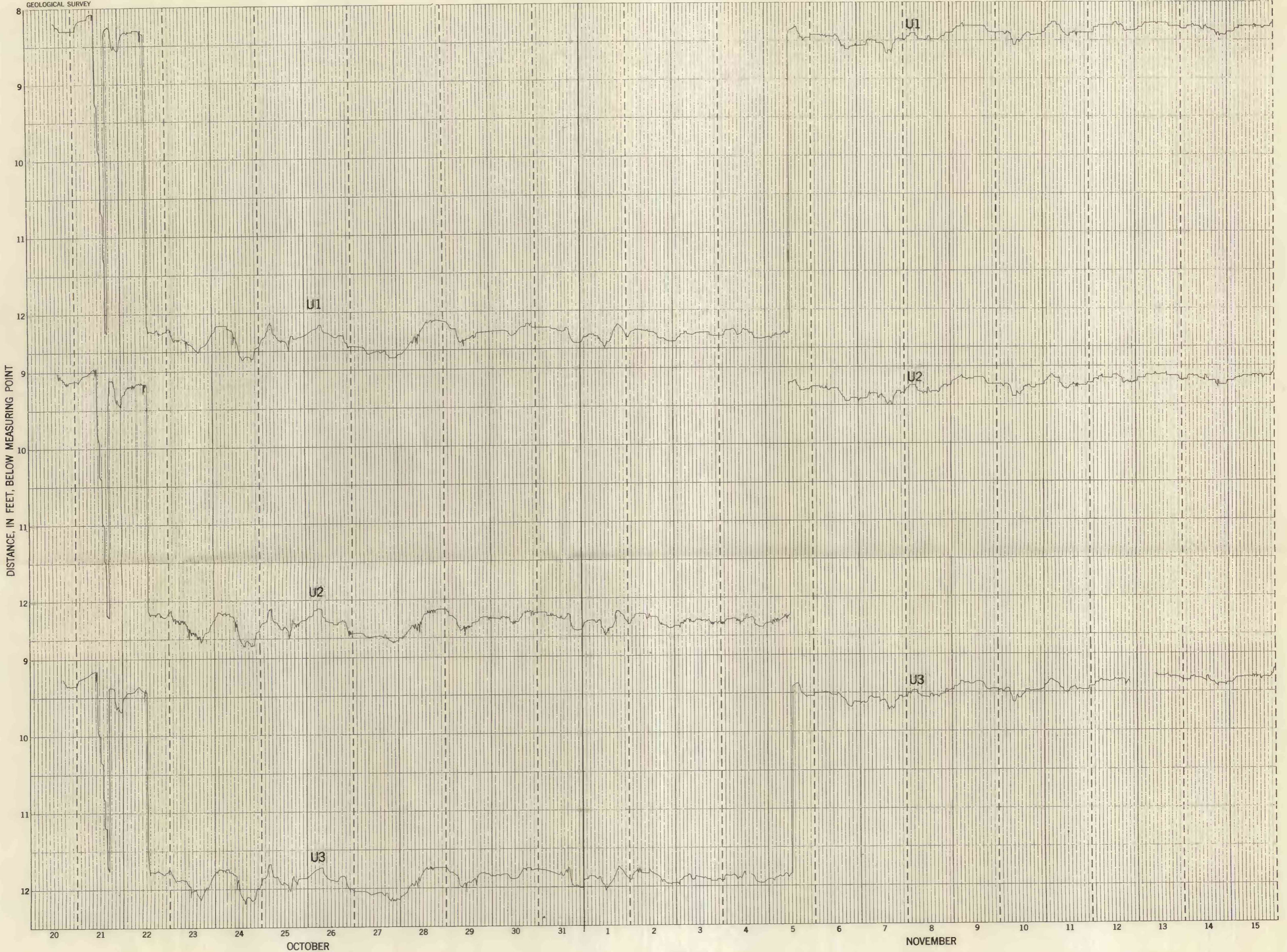
GRAPHS OF WATER LEVEL IN OBSERVATION WELLS U1, U2, AND U3 DURING PUMPING TEST IN NORTHEASTERN SECTION OF LOUISVILLE AREA, 1946
