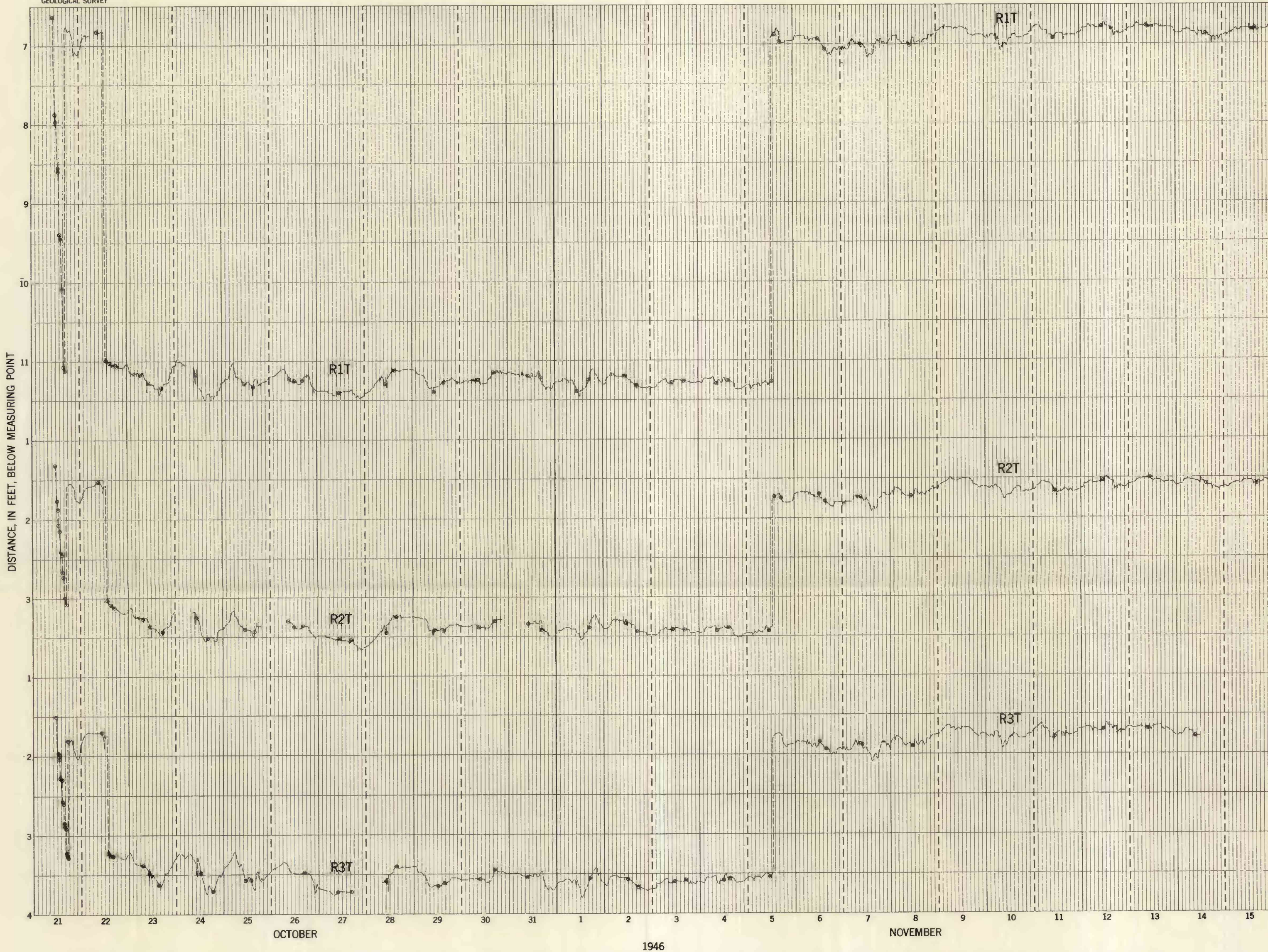
GRAPHS OF WATER LEVEL IN OBSERVATION WELLS R1T, R2T, AND R3T DURING PUMPING TEST IN NORTHEASTERN SECTION OF LOUISVILLE AREA, 1946
