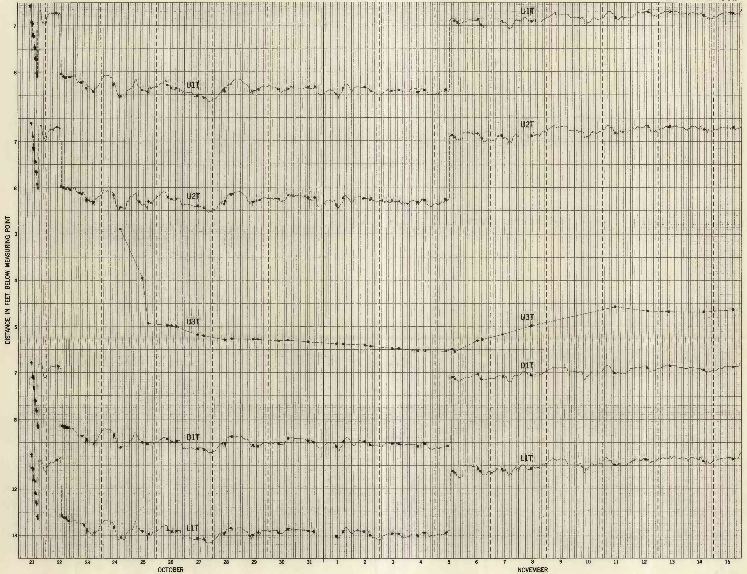
GRAPHS OF WATER LEVEL IN OBSERVATION WELLS U1T, U2T, U3T, D1T AND L1T, DURING PUMPING TEST IN NORTHEASTERN SECTION OF LOUISVILLE AREA, 1946
