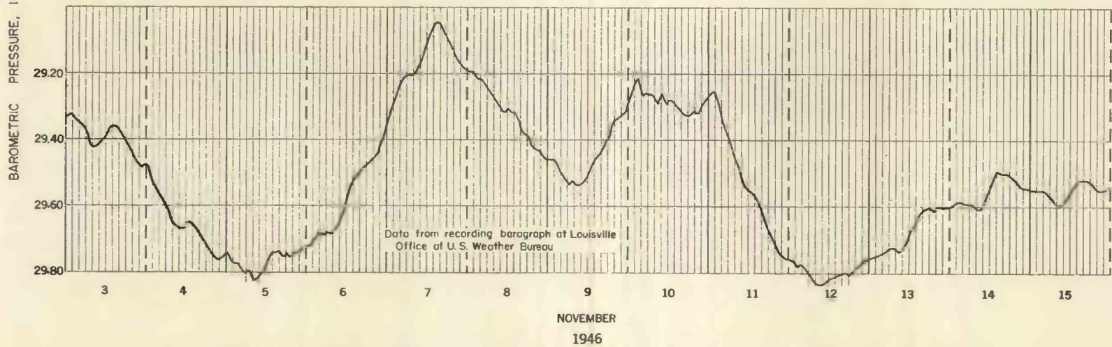
GRAPH OF BAROMETRIC PRESSURE DURING PUMPING TEST, 1946
