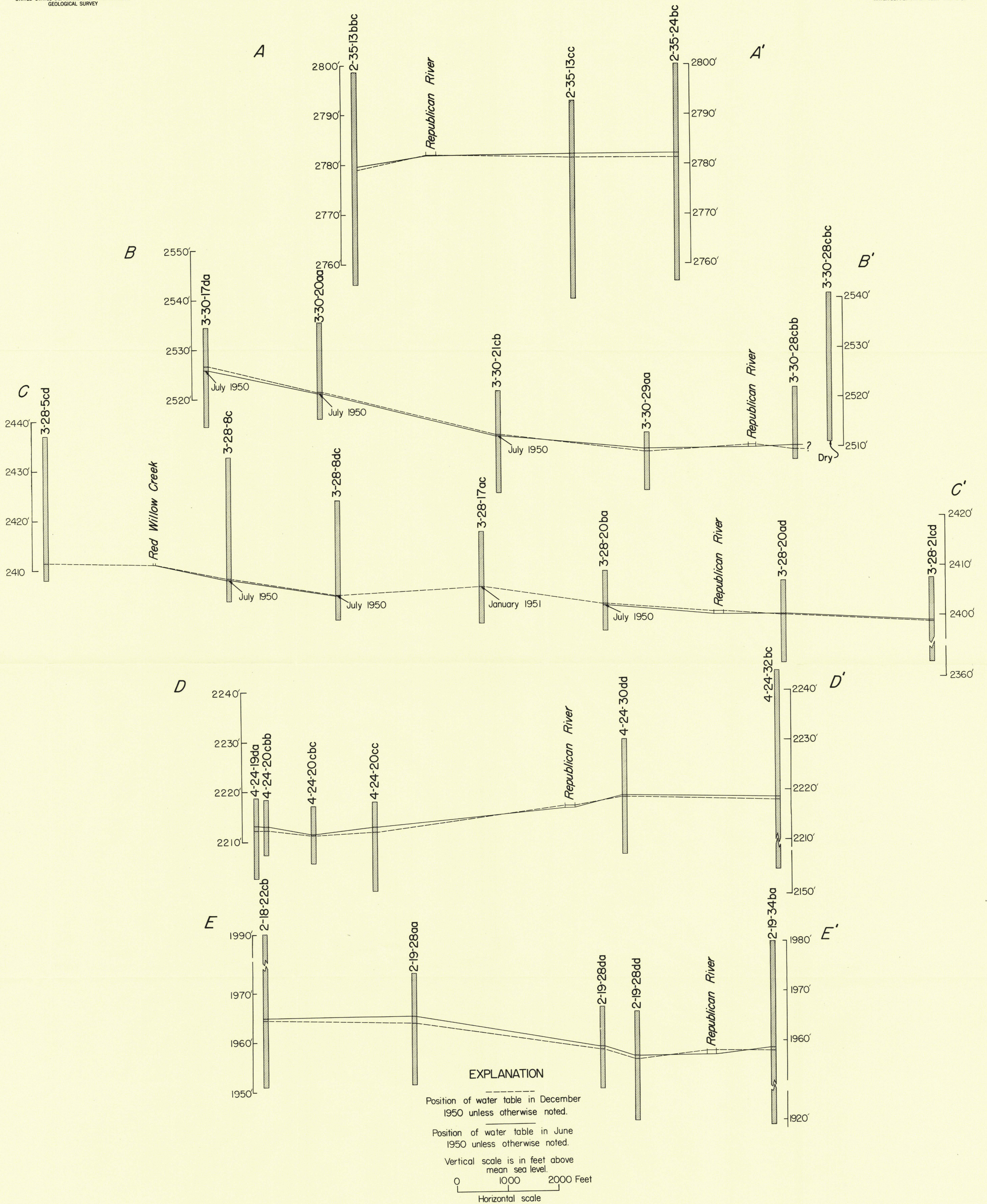
PROFILES OF THE WATER TABLE IN THE REPUBLICAN RIVER VALLEY, NEBRASKA
