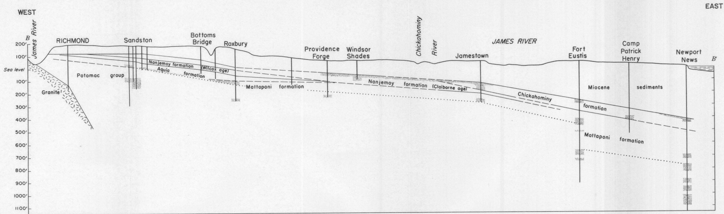
GEOLOGIC CROSS SECTIONS OF THE YORK-JAMES PENINSULA, VIRGINIA
