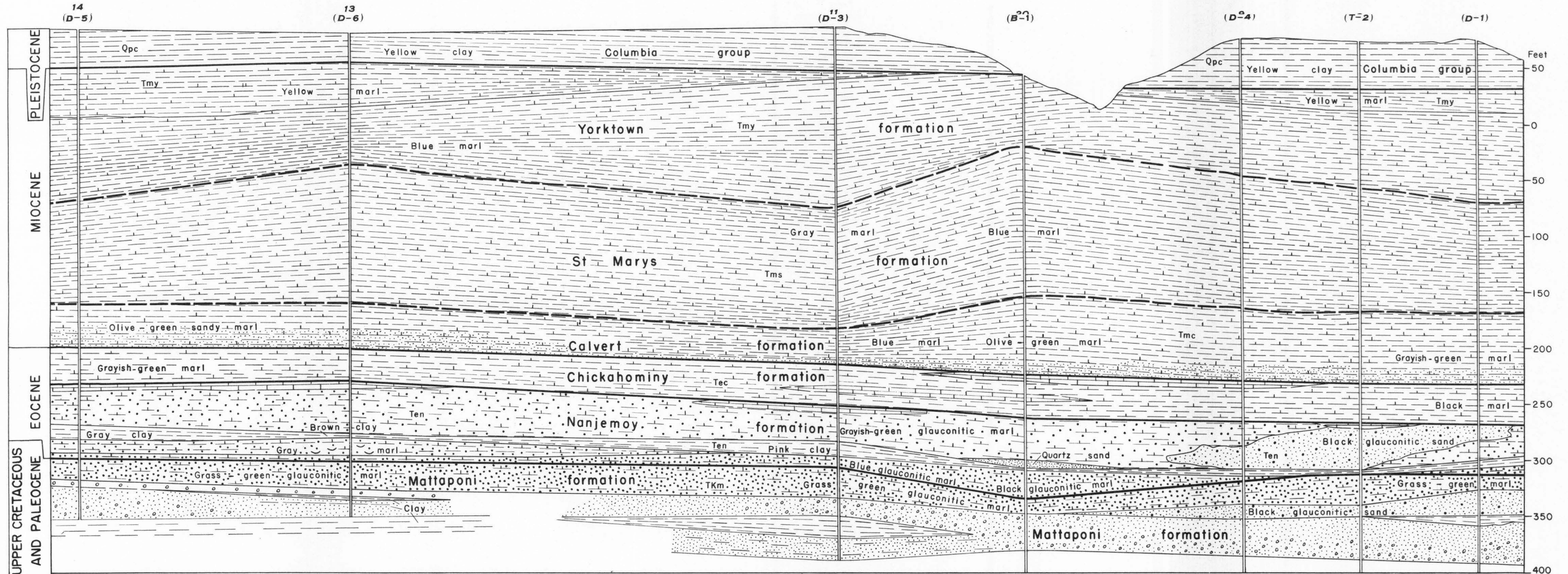
GEOLOGIC CROSS SECTION THROUGH WELLS AT CAMP PEARY, YORK COUNTY, VIRGINIA
