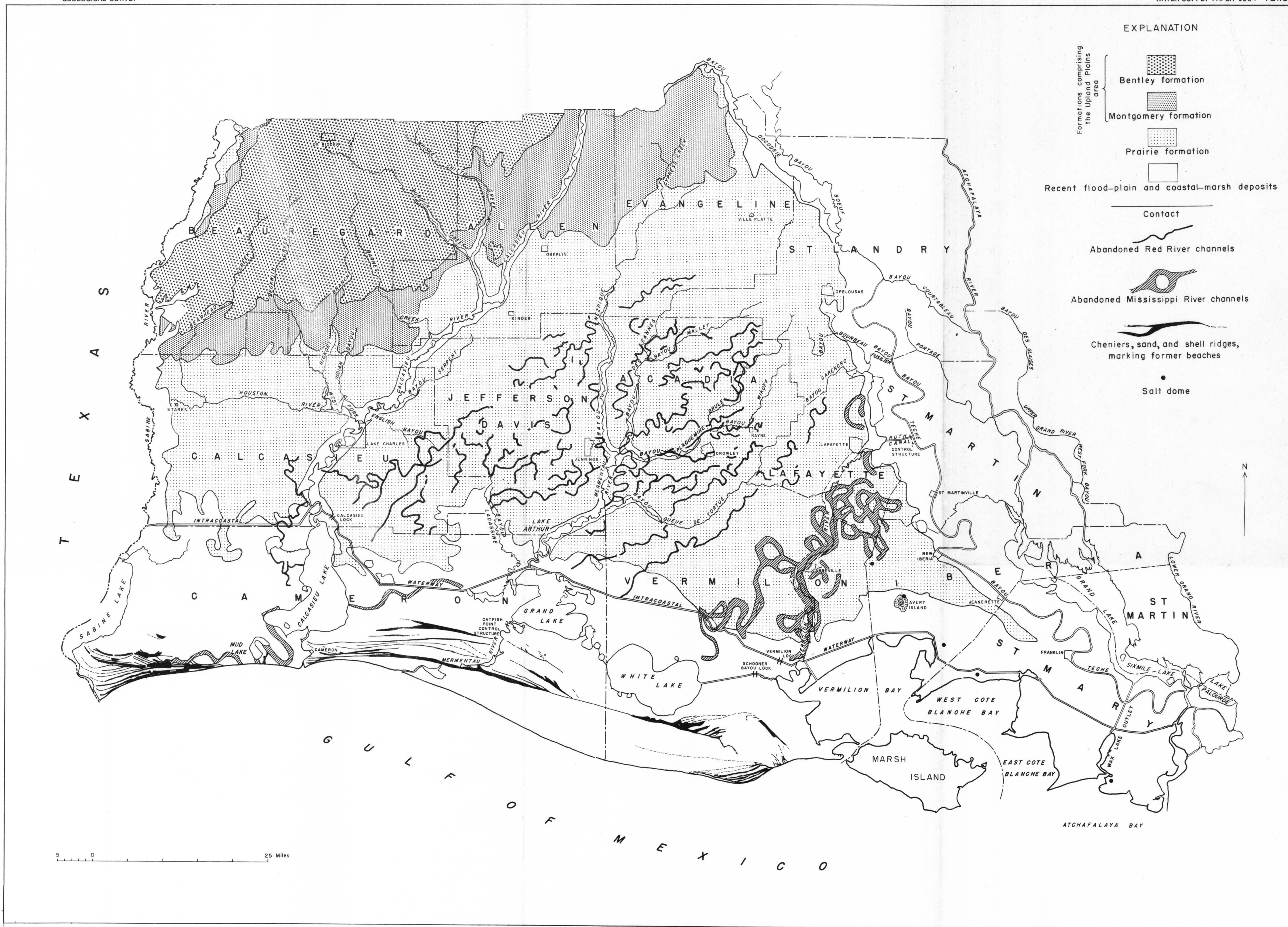
GEOLOGIC AND PHYSIOGRAPHIC MAP OF SOUTHWESTERN LOUISIANA
