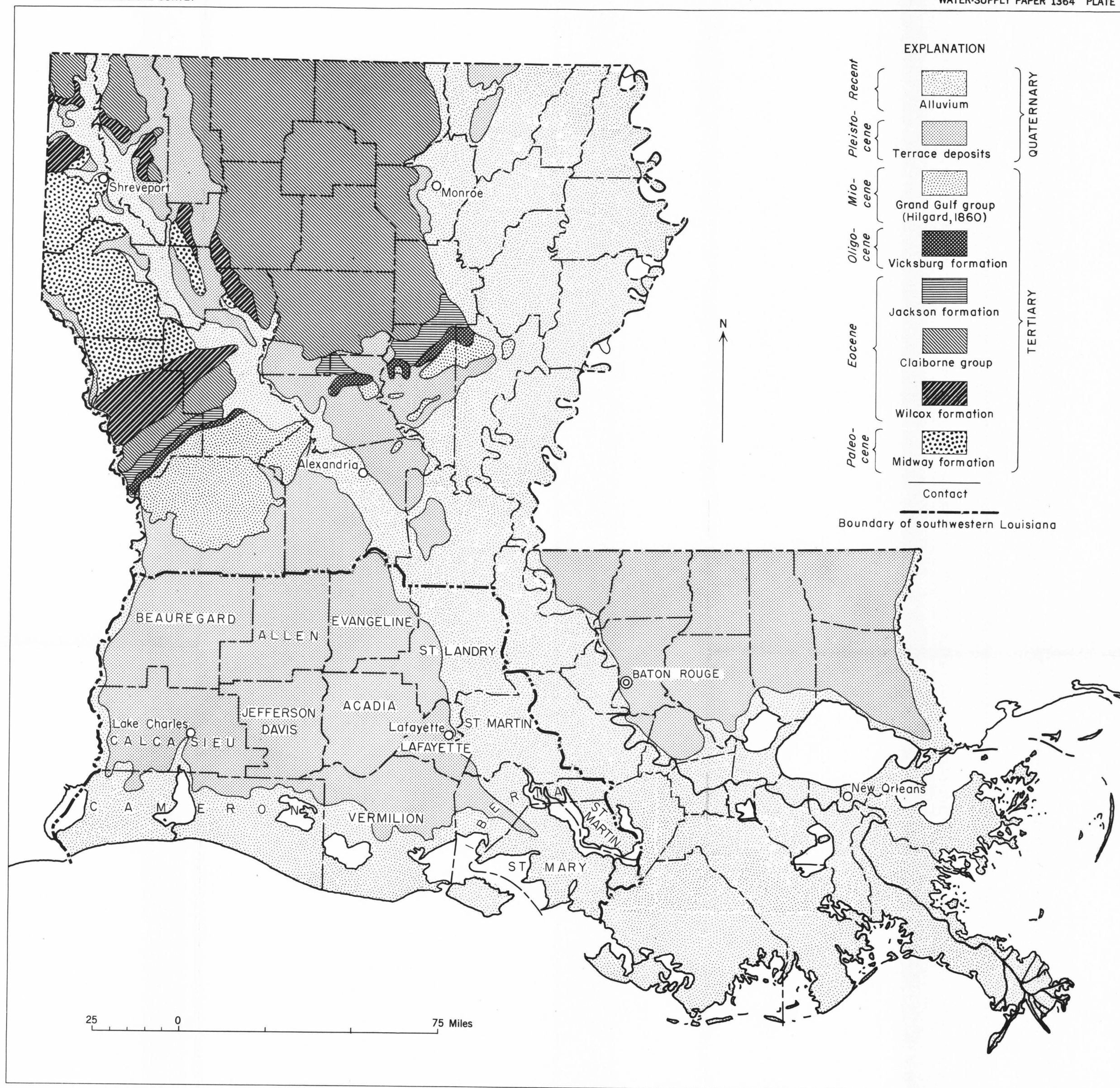
GENERALIZED GEOLOGIC MAP OF LOUISIANA
