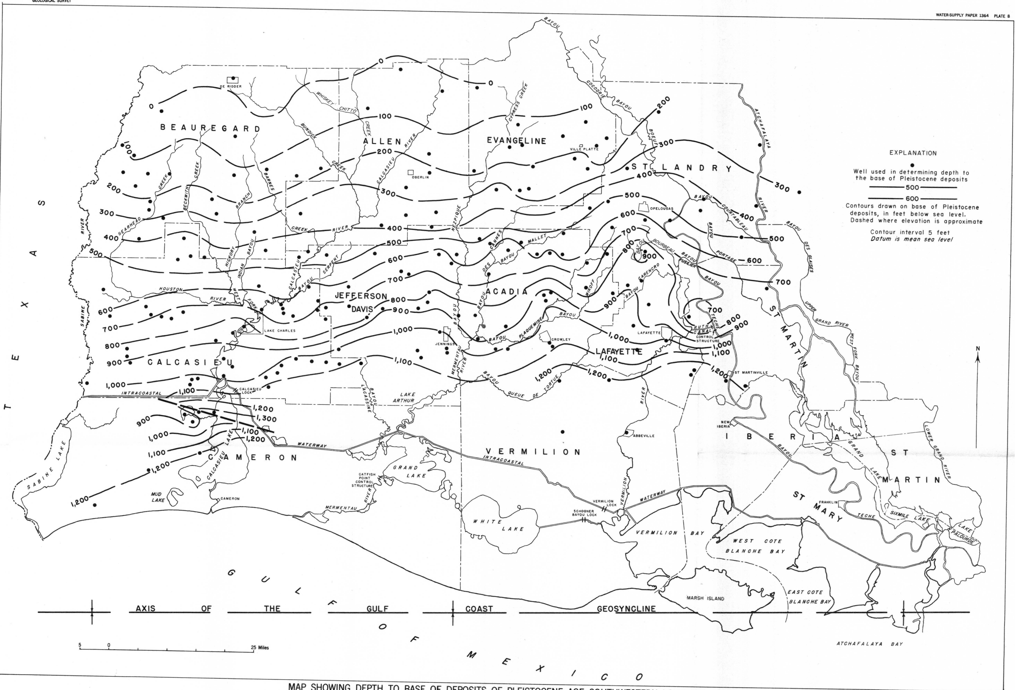
MAP SHOWING DEPTH TO BASE OF DEPOSITS OF PLEISTOCENE AGE, SOUTHWESTERN LOUISIANA
