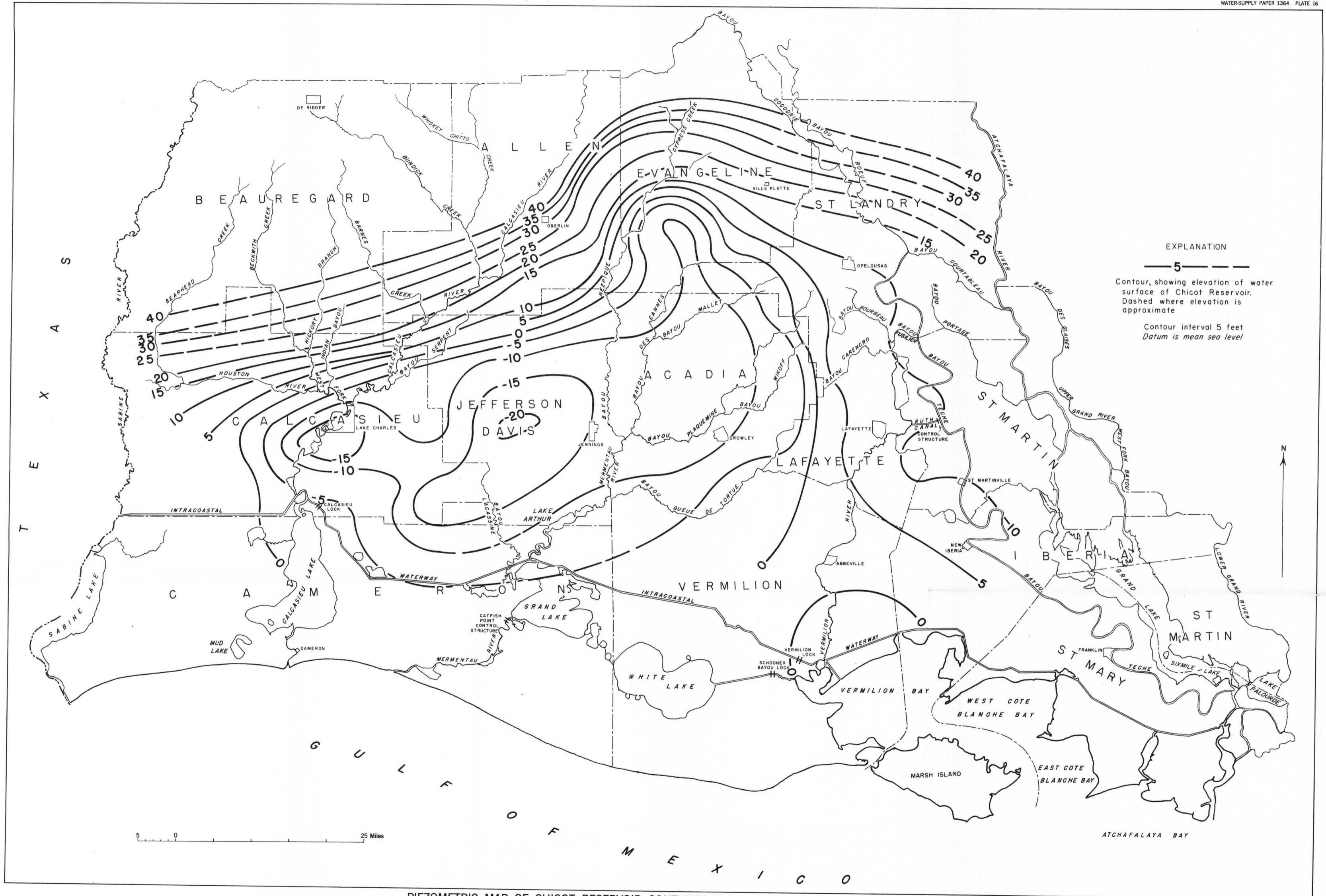
PIEZOMETRIC MAP OF CHICOT RESERVOIR, SOUTHWESTERN LOUISIANA, SEPTEMBER 1944
