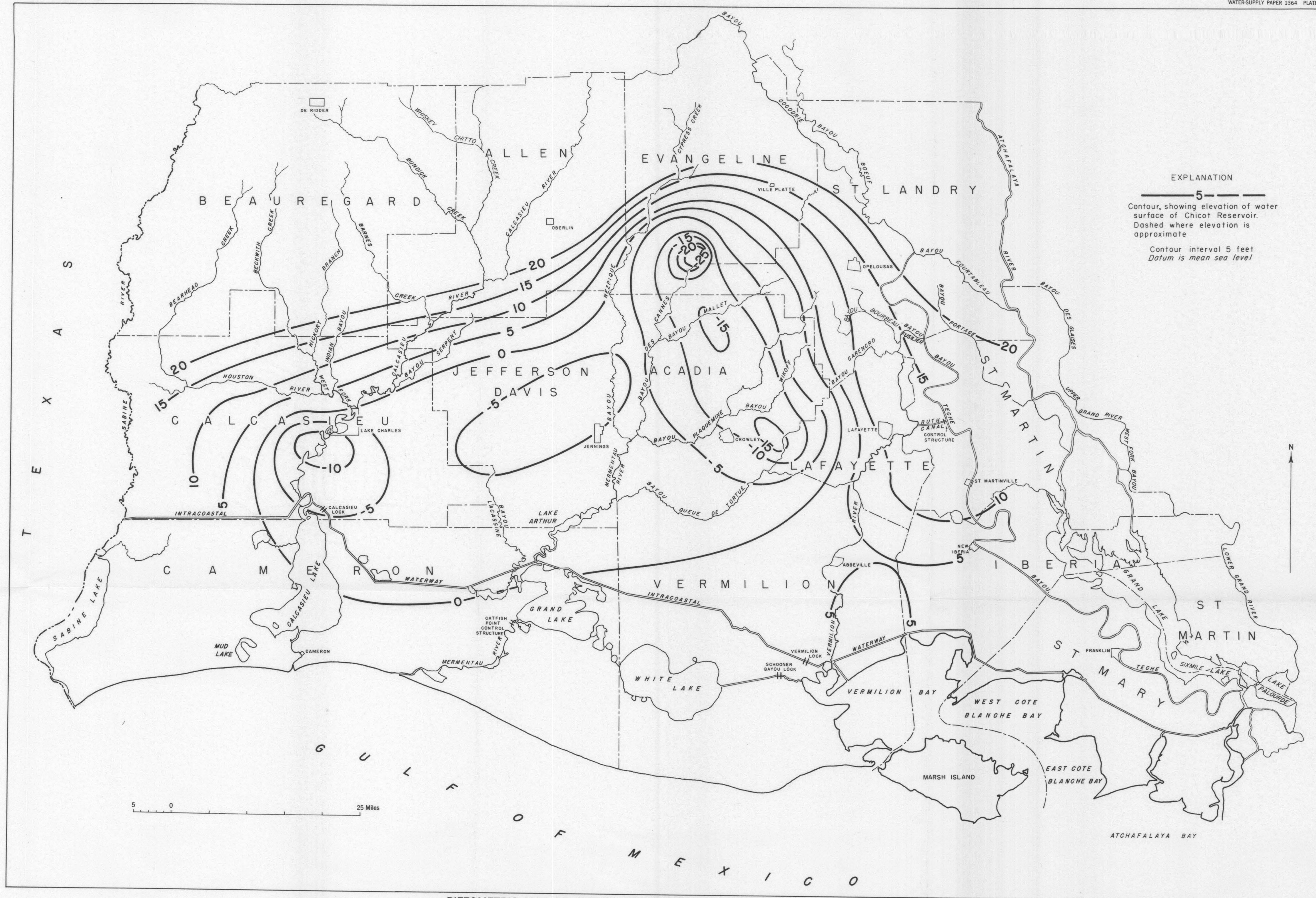
PIEZOMETRIC MAP OF CHICOT RESERVOIR, SOUTHWESTERN LOUISIANA, MAY 1947
